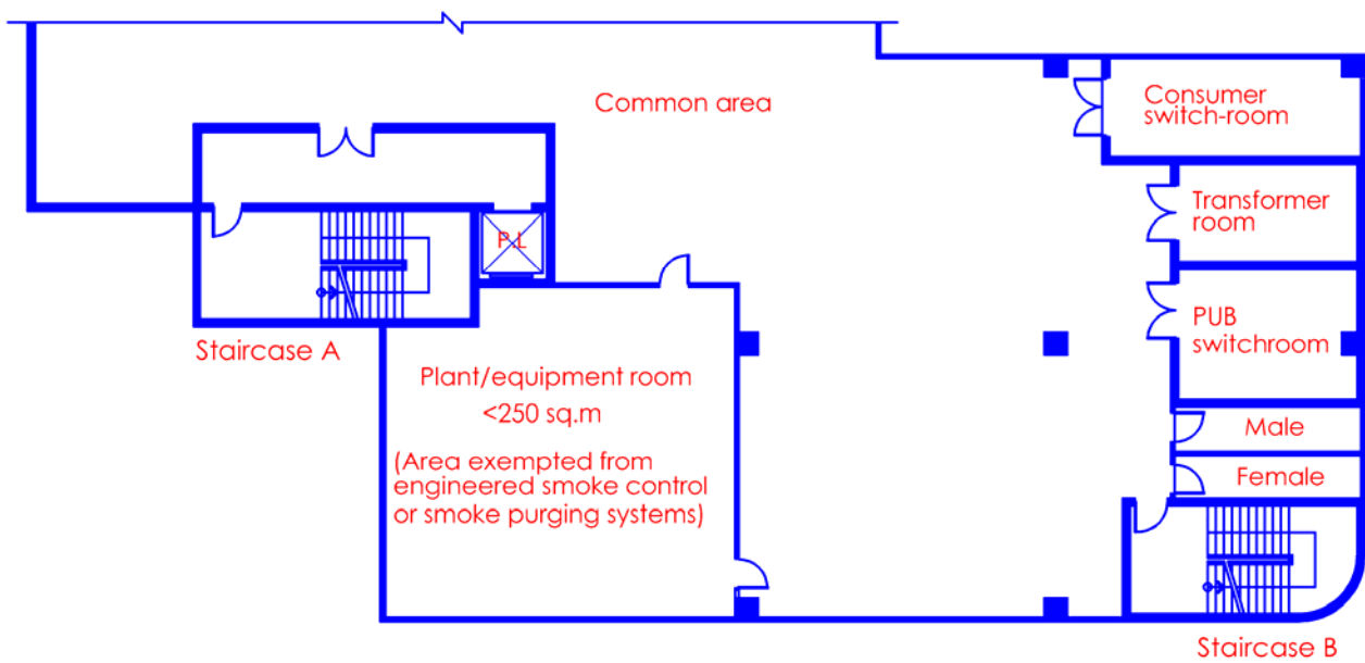
Part plan of basement storey
