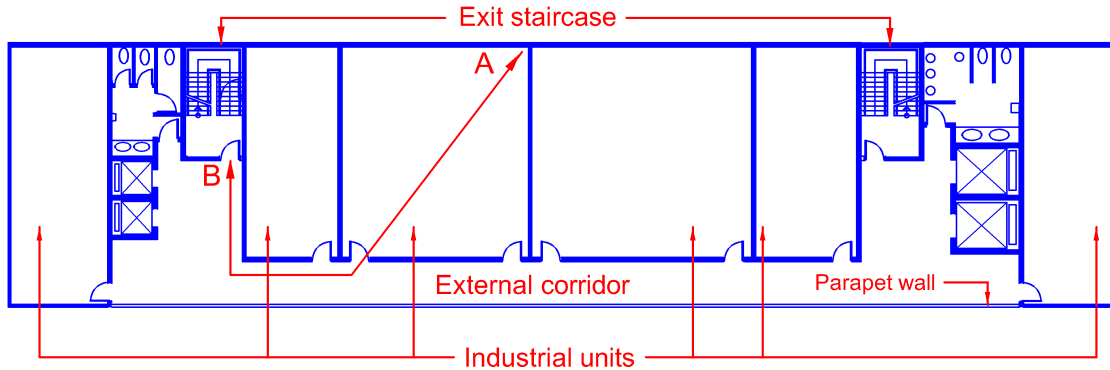
Diagram 2.2.13(a)(iii)-4
