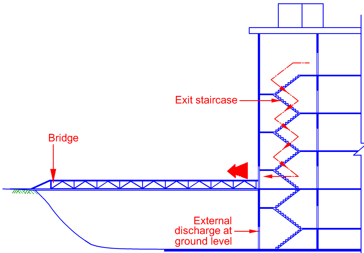
Diagram 2.3.3(c)(i)-3
