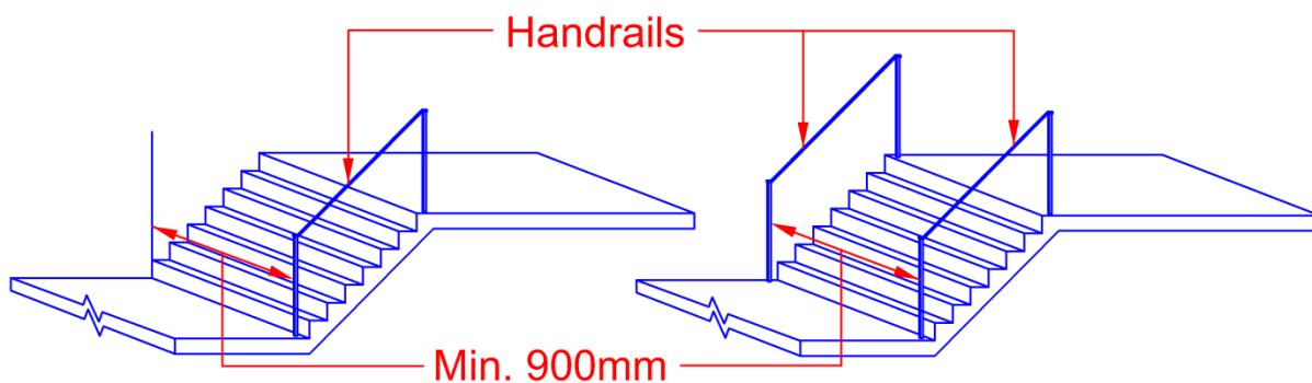
Diagram 2.2.1
