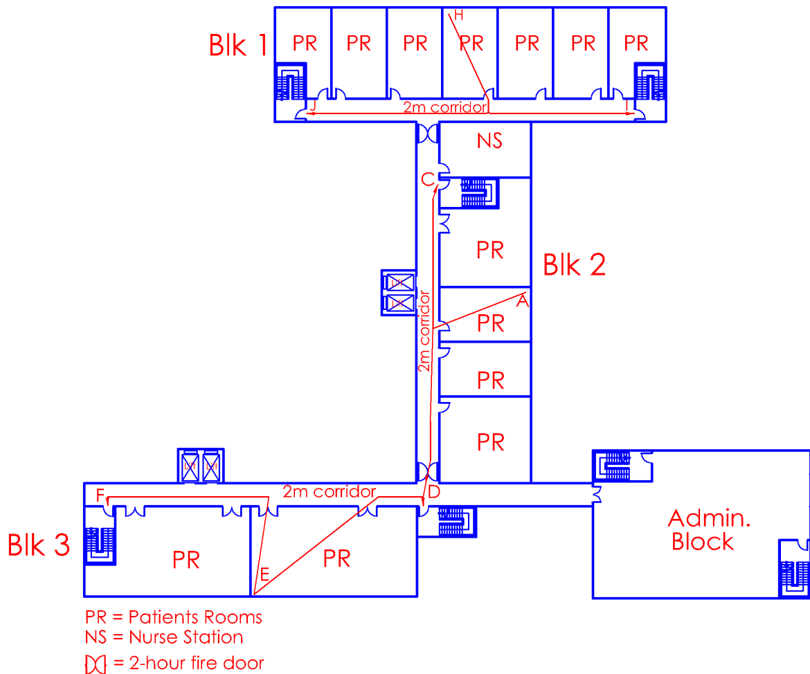
Diagram 2.5.1(a)
