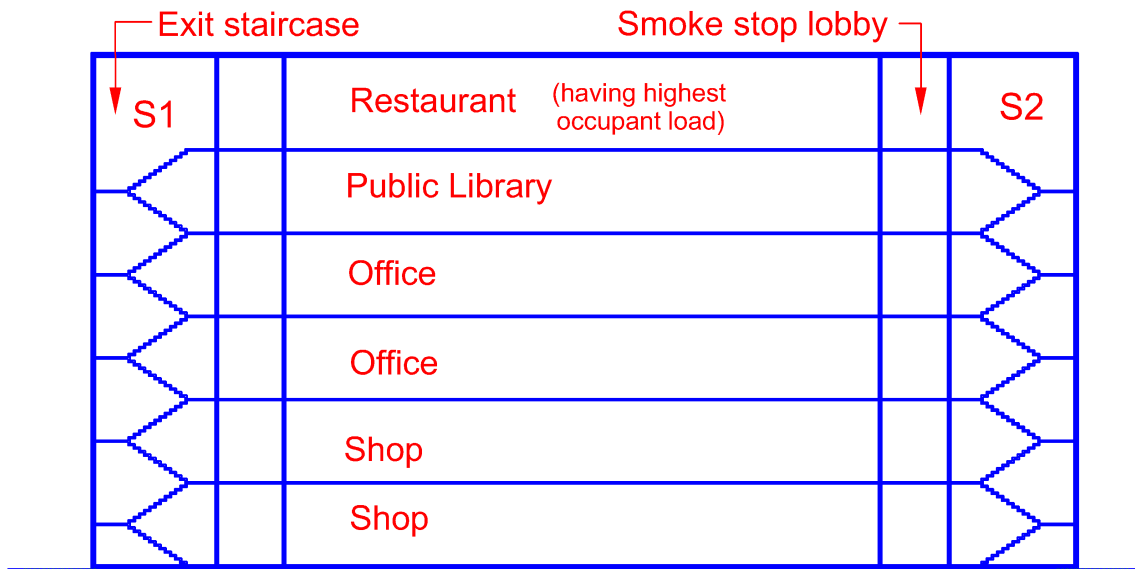
Diagram 2.2.2-10
