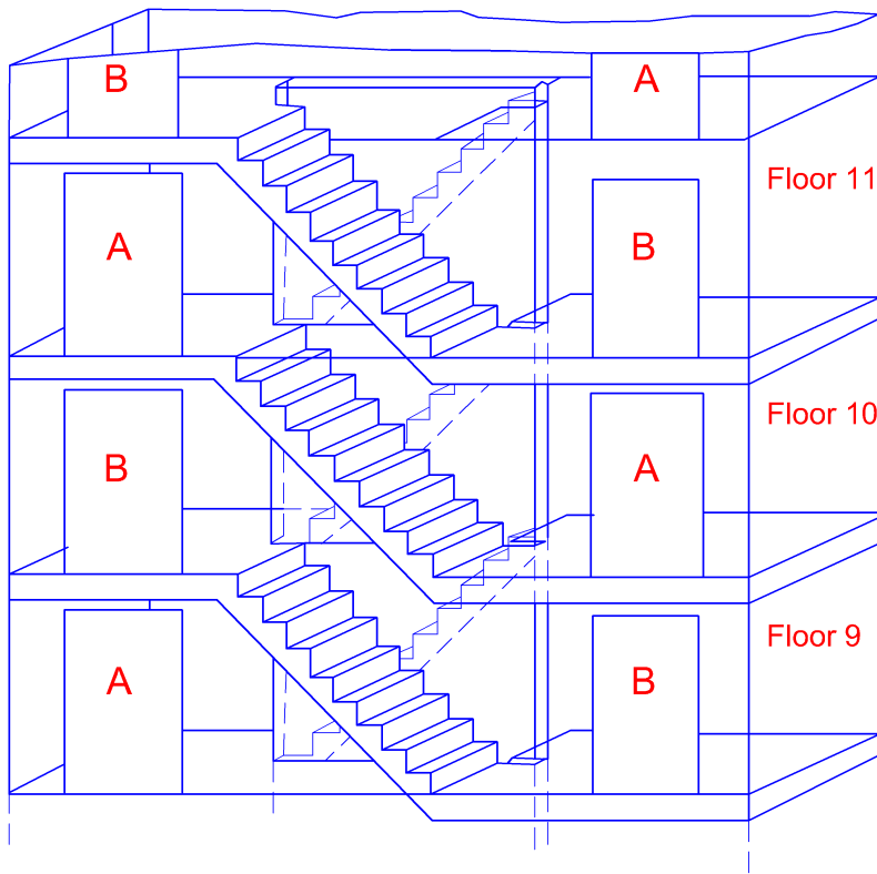
Scissors stairs.
