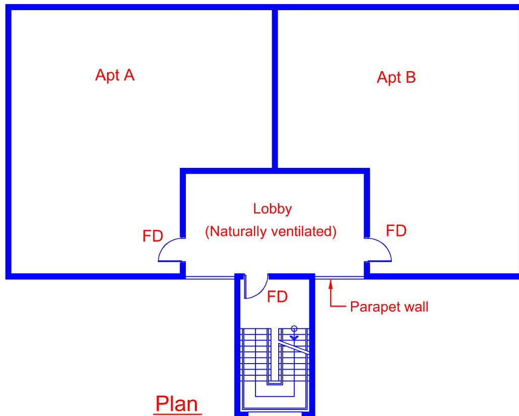
Diagram 2.4.4-2
