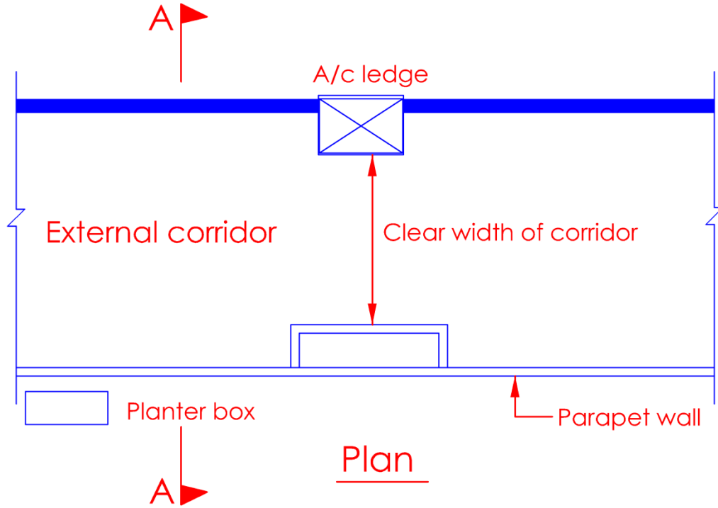
Diagram 2.2.7-5
