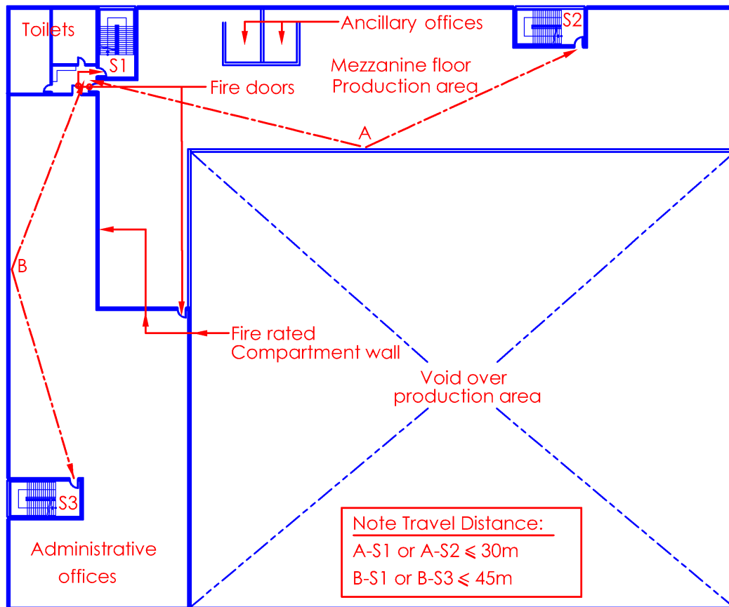
Diagram 2.2.6(h)
