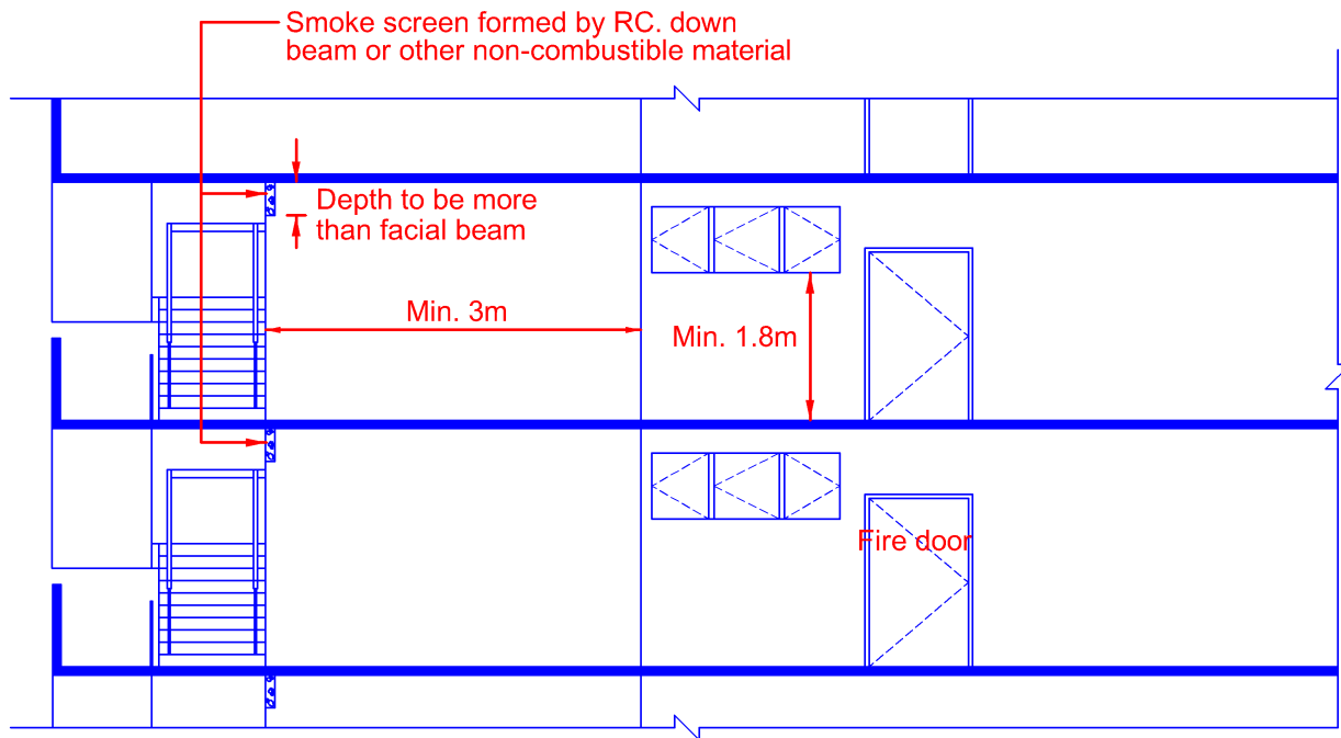
Diagram 2.2.13(a)(iii)-3
