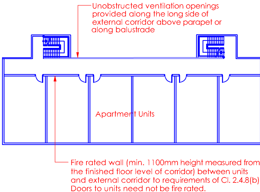
Diagram 2.3.3(b)(ii)-4
