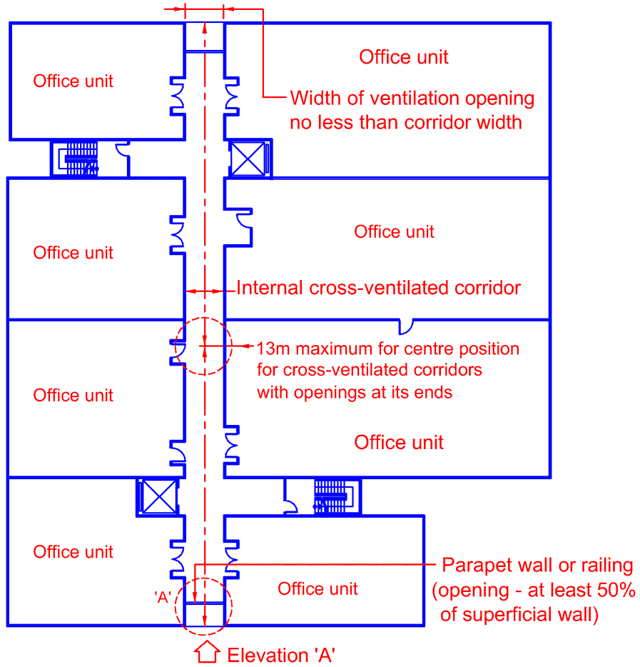
Diagram 2.2.13(b)(iv)-2
