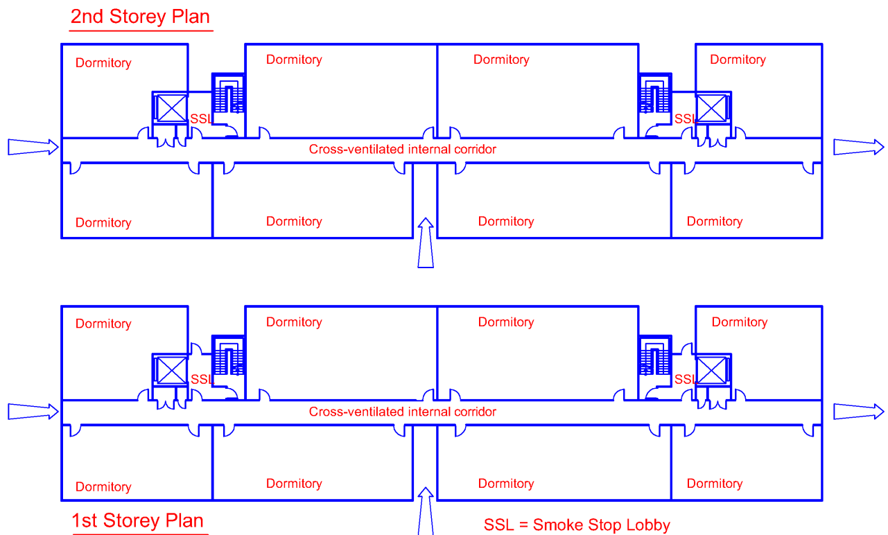
Diagram 2.9.5
