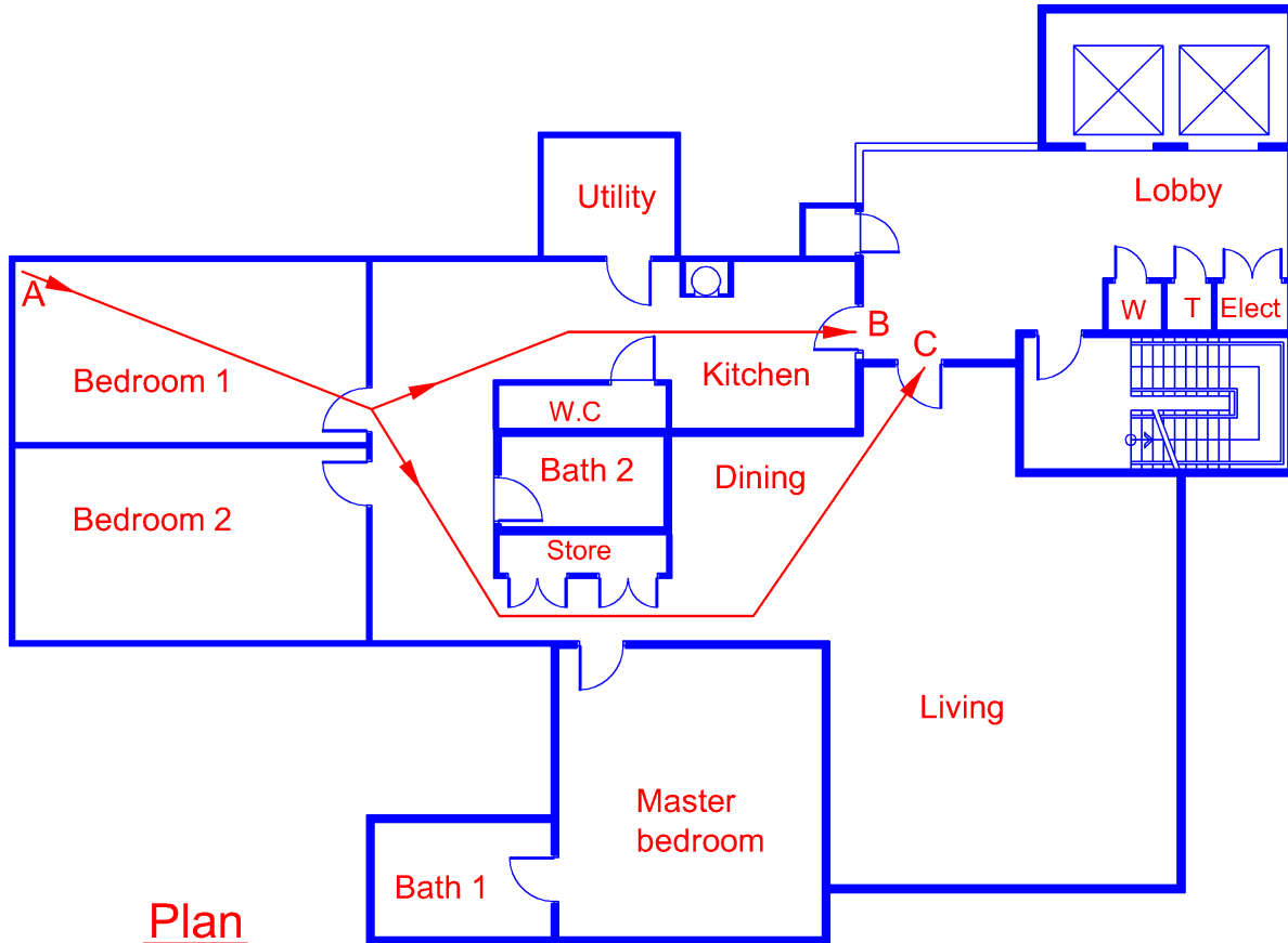
Diagram 2.4.6(a)-2
