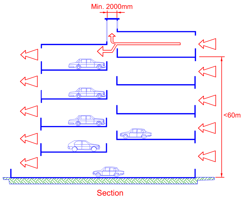
Open-sided multi-storey car park
