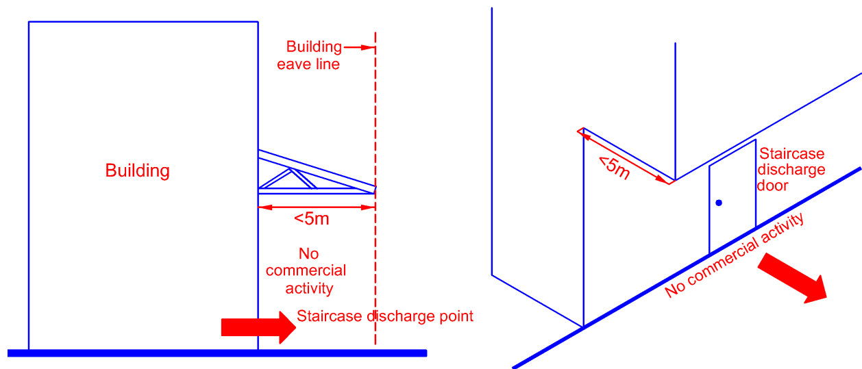
Diagram 2.3.3(c)(i)-1
