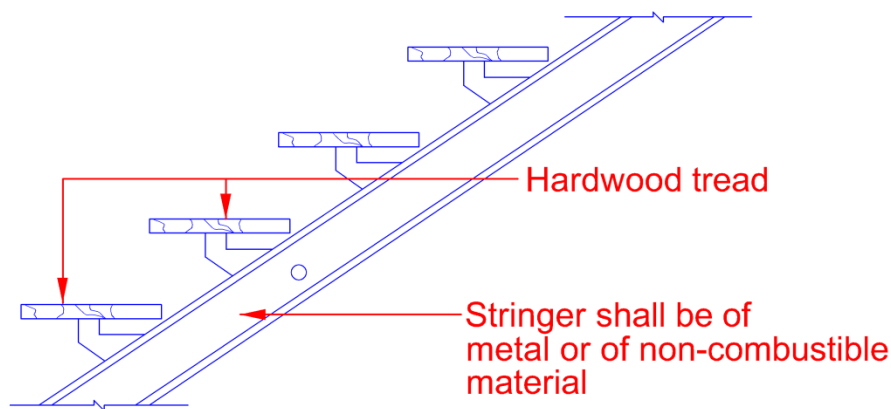
Unenclosed staircase
