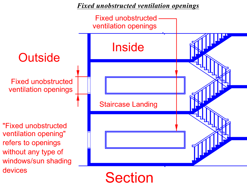
Diagram 2.2.13(c)(ii)-8
