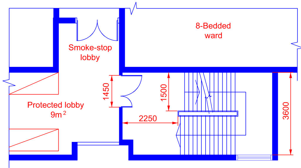
Diagram 2.5.1 (a)(ix)
