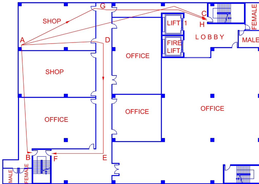
AB and AC are Direct Distance measurement paths annotated by \longleftrightarrow ADEF and AGH are Travel Distance measurement paths annotated by \longleftrightarrow
