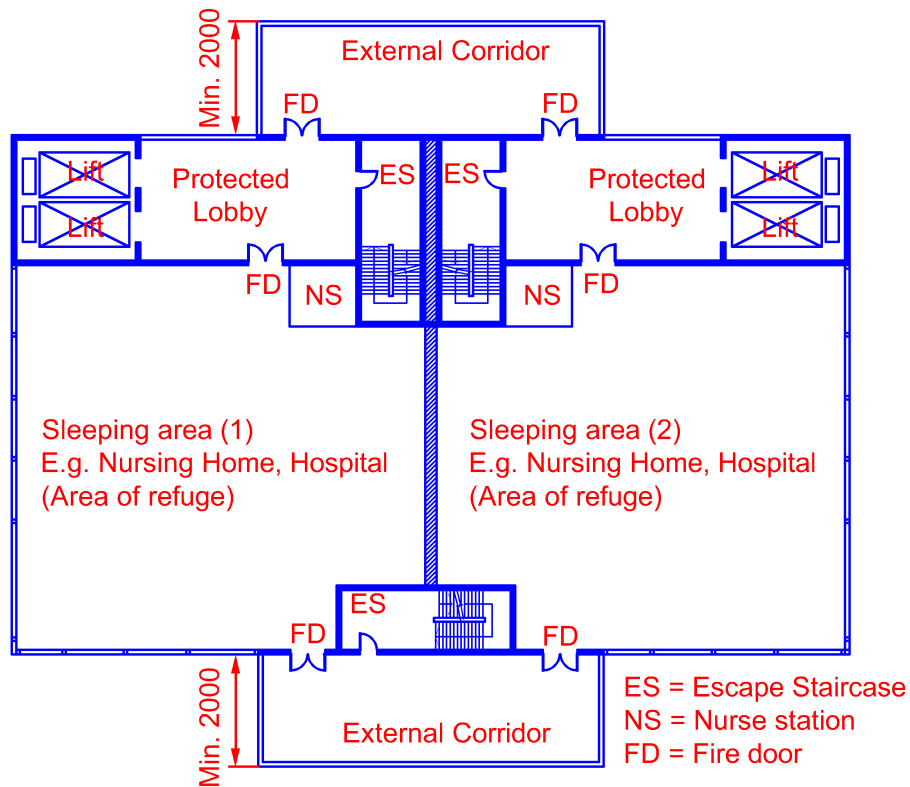
Example (1) of health care occupancy layout
