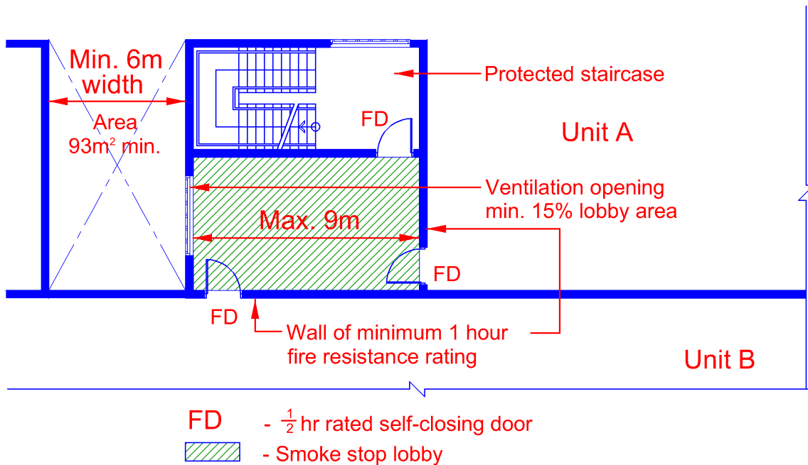
Diagram 2.2.13(b)(i)-1
