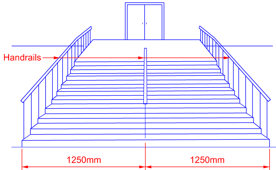
Diagram 2.2.8-2
