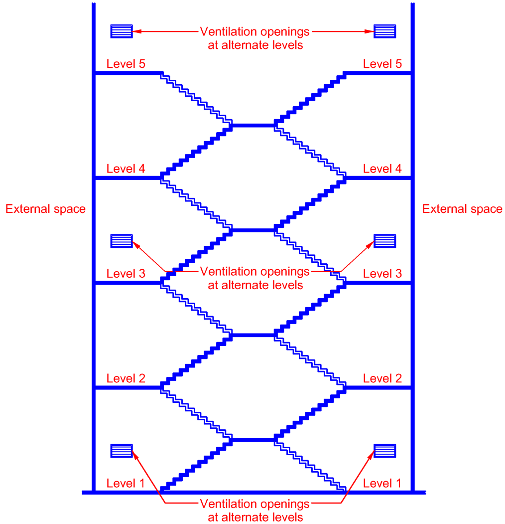
Diagram 2.3.4(e)-1
