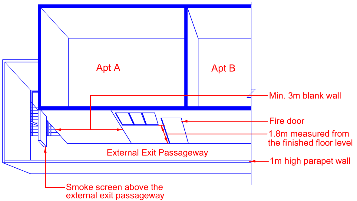
Diagram 2.2.13(a)(iii)-2
