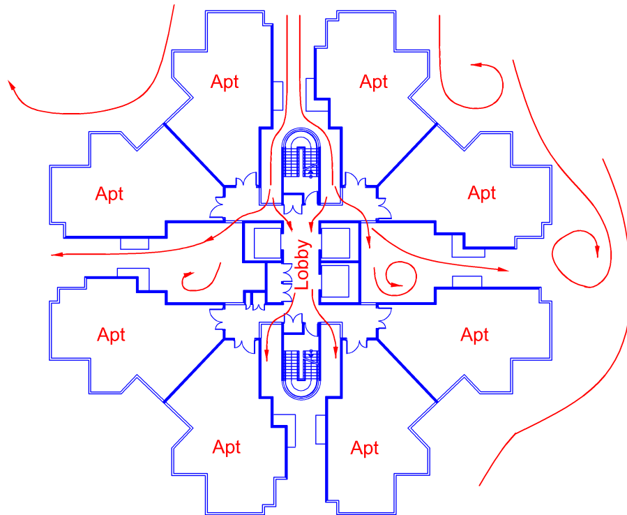
Diagram 2.4.8 (a) & (b)-3
