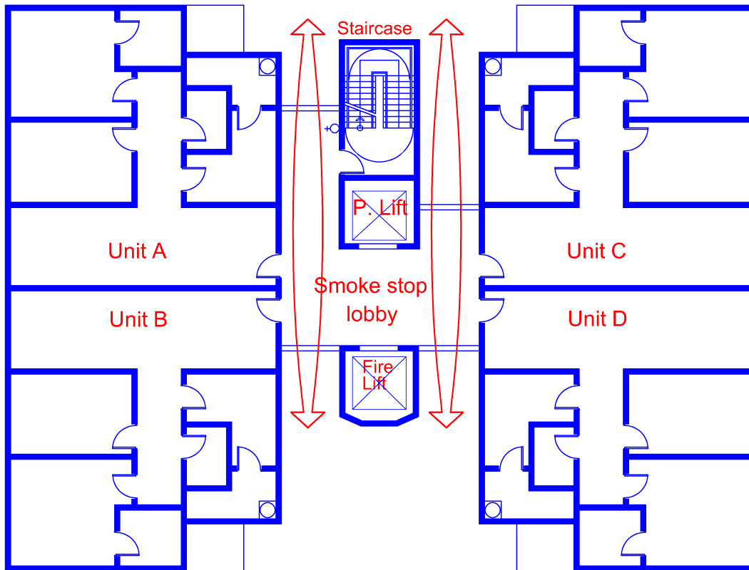
Diagram 2.2.13(b)(i)-2
