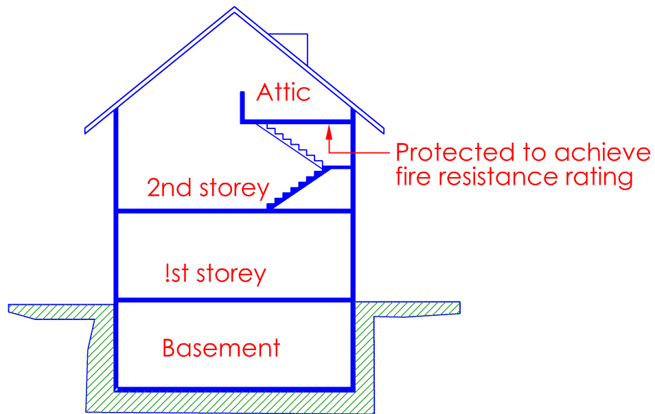
Diagram 2.4.12
