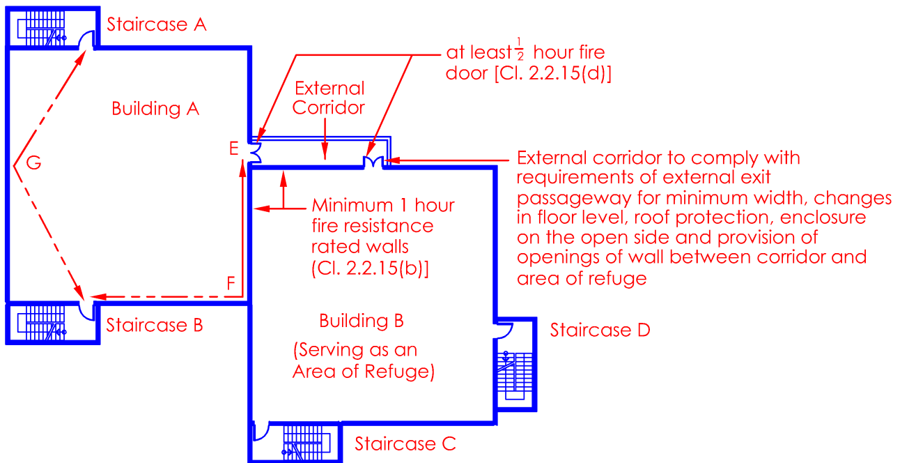
Diagram 2.2.6(f)-3
