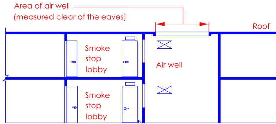
Sectional view
