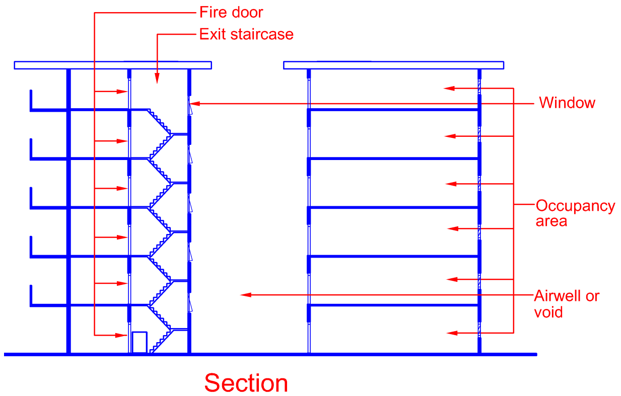
Diagram 2.3.3(f)-1
