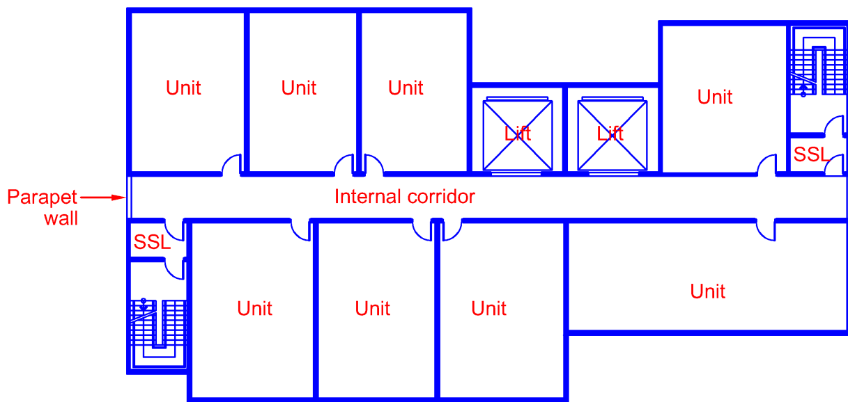
Diagram 2.4.13
