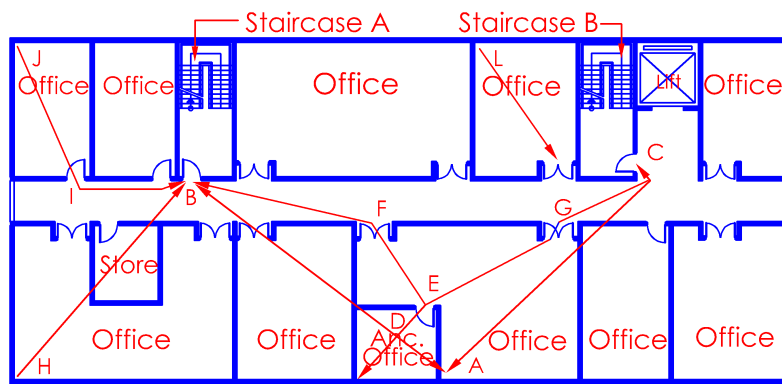
Typical Storey Plan of Office Building
