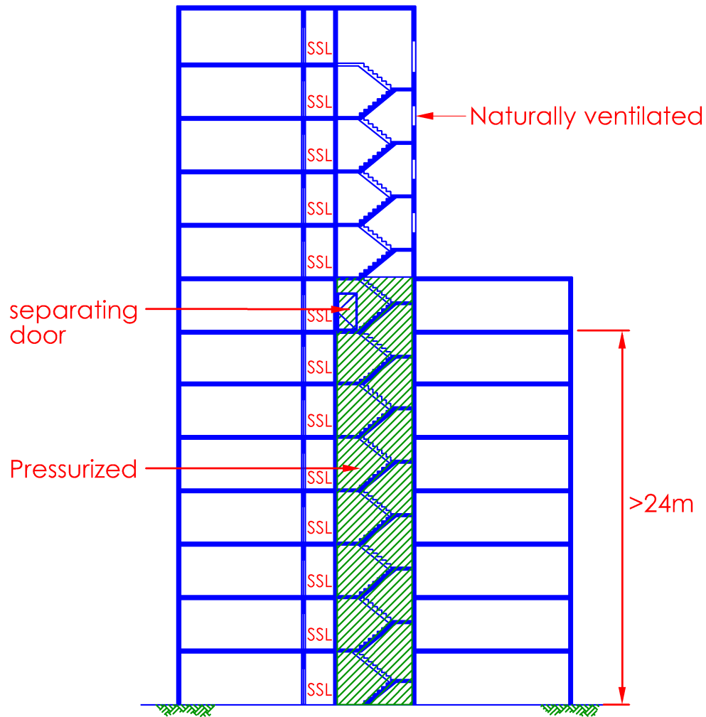
Diagram 2.3.3(h)-2
