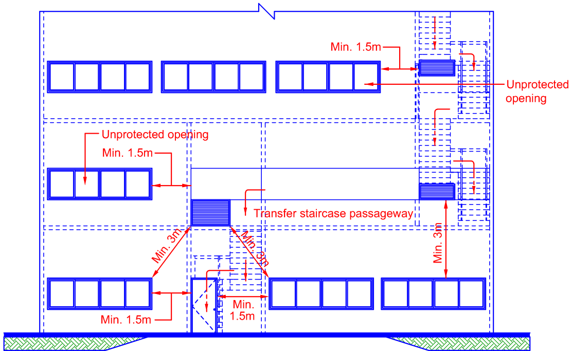
Diagram 2.3.3(a)(iii)-2
