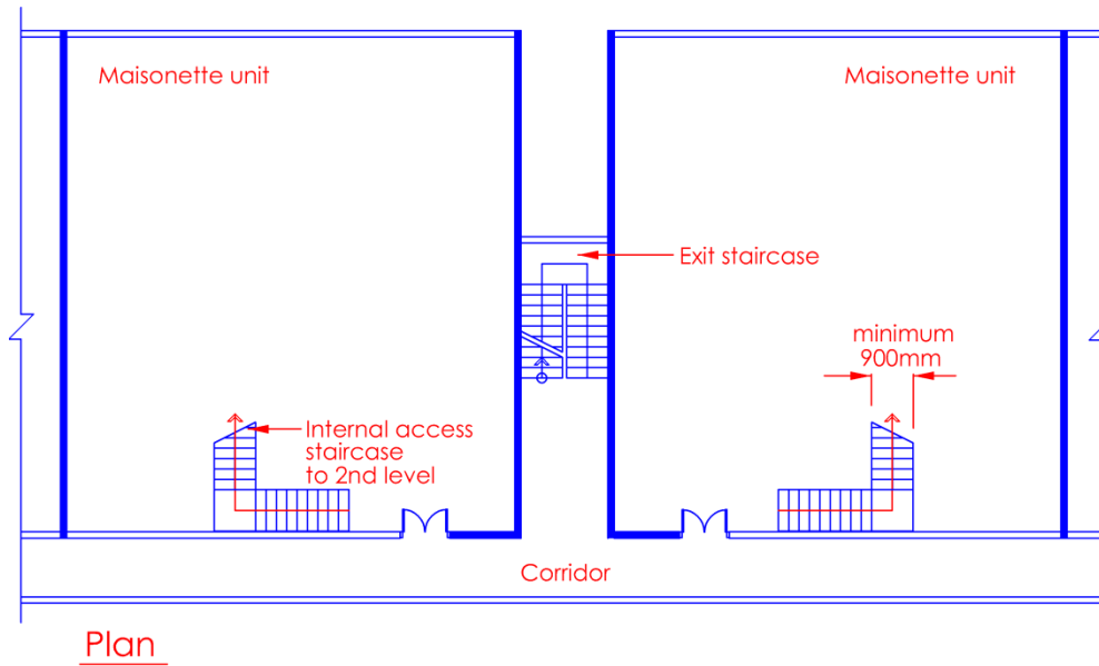
Diagram 2.2.7-9
