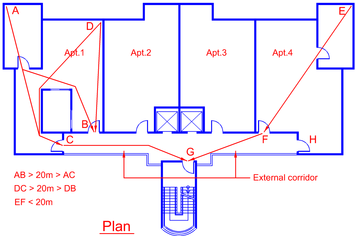
Diagram 2.4.7-1
