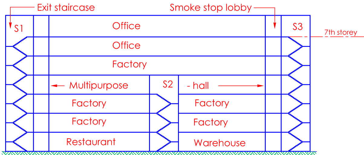
Diagram 2.2.3-2
