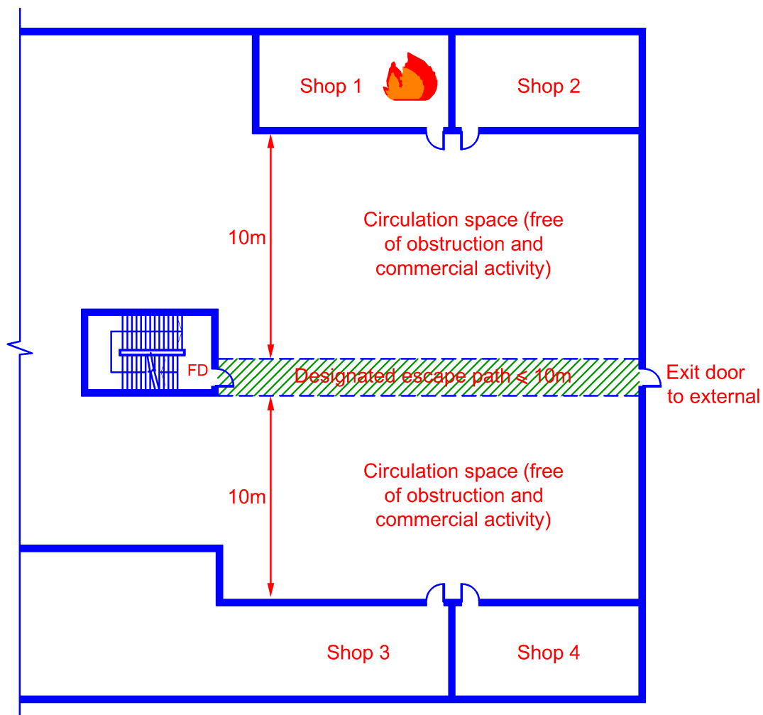
Diagram 2.3.3(c)(i)-4
