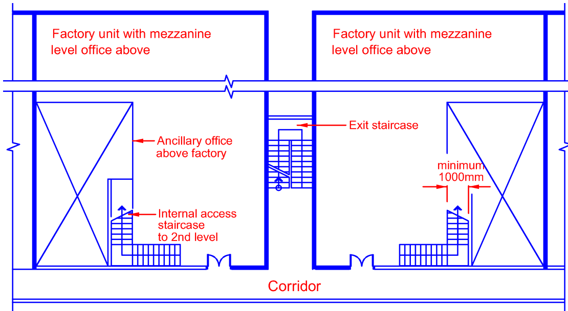
Diagram 2.2.7-10
