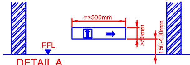
DETAIL A PL TAPE WITH DIRECTIONAL ARROW & EXIT LEGEND ON STAIRCASE LANDING WALL
