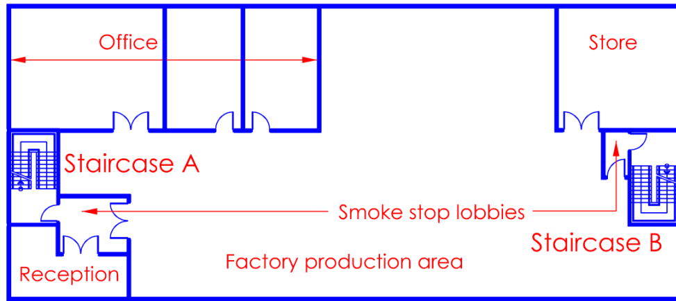
Diagram 2.2.11
