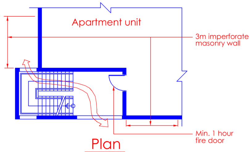
Diagram 2.2.13(c)(i)(3) & 2.2.13(c)(ii)
