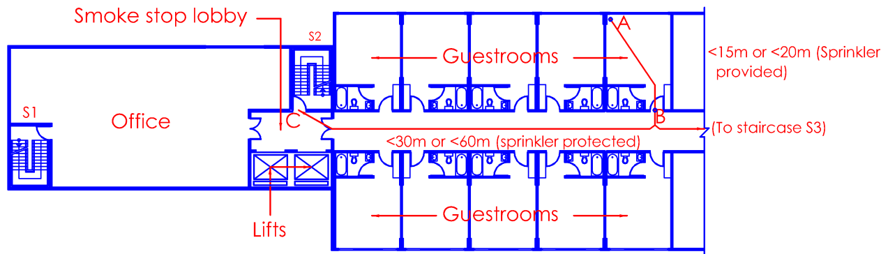
Diagram 2.2.2 – 8
