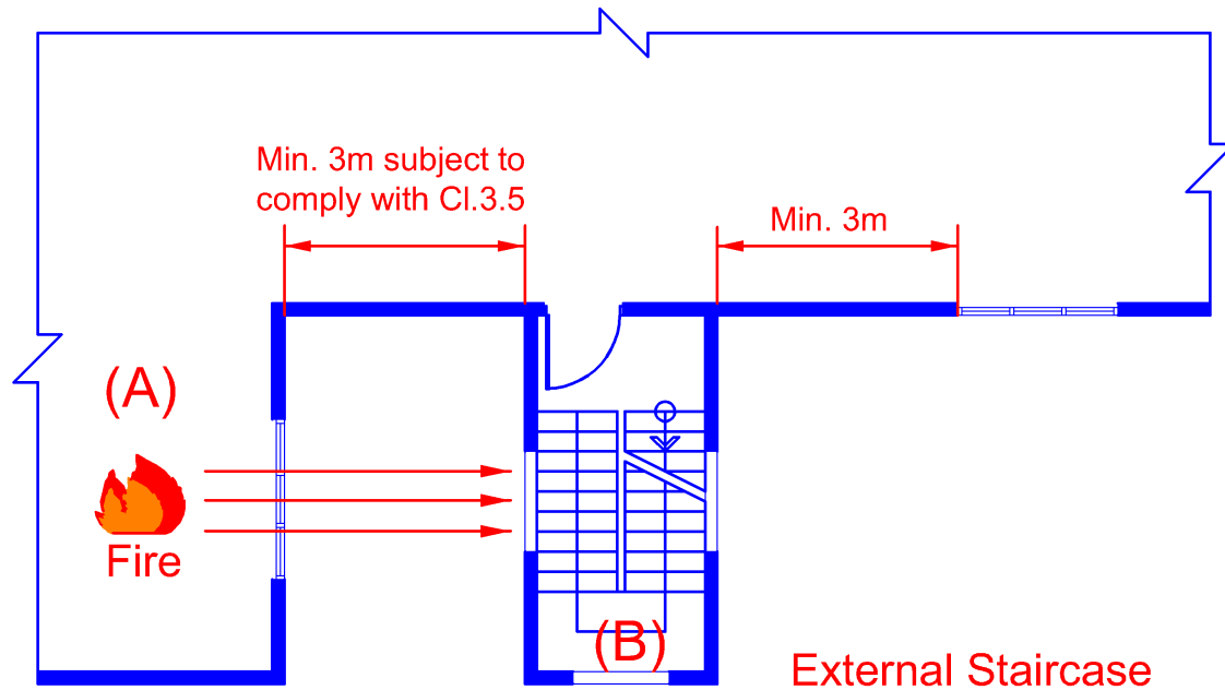
Diagram 2.3.3(b)(ii)-2
