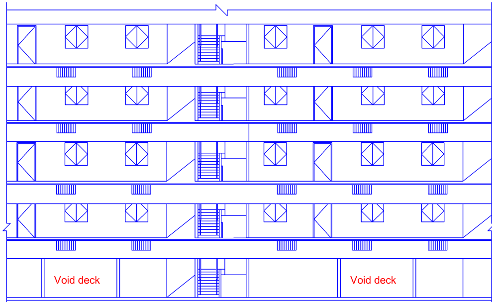
Elevation view
