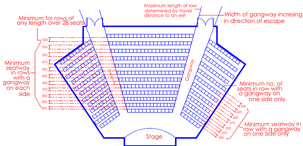
Diagram 2.8.3(a)-2
