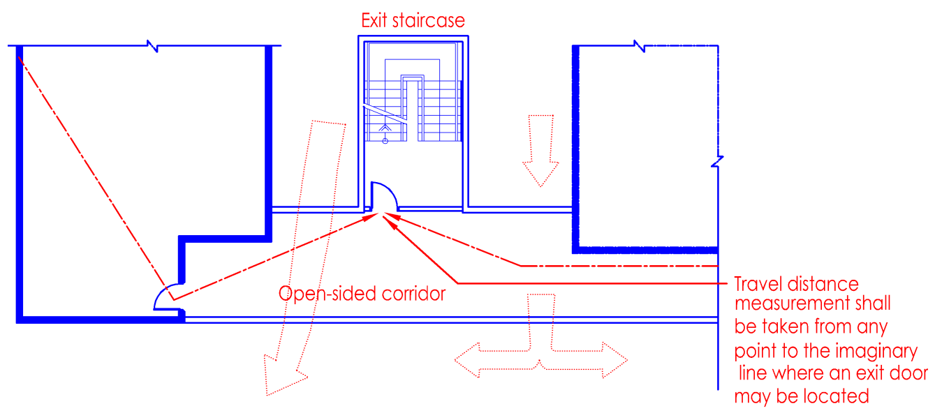
Diagram 2.2.6(g)
