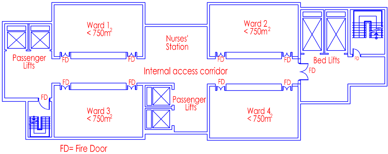
Diagram 2.5.1 (a)(iv)
