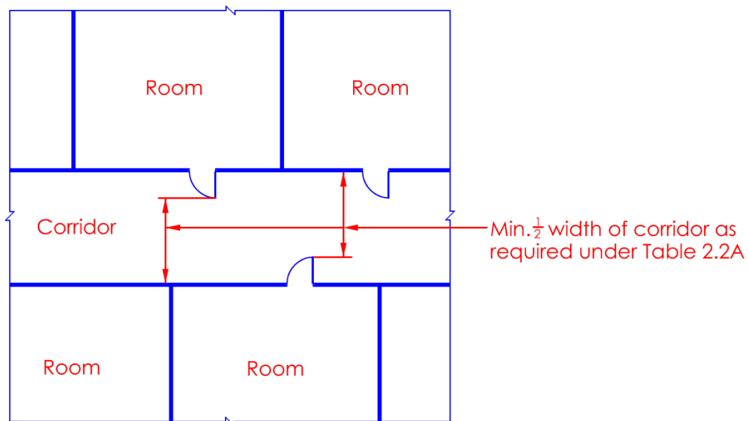
Diagram 2.2.7-2
