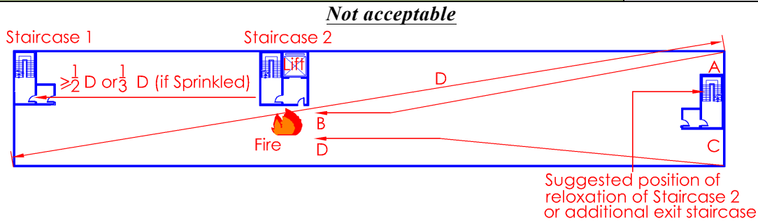
Diagram 2.2.6(a)-1
