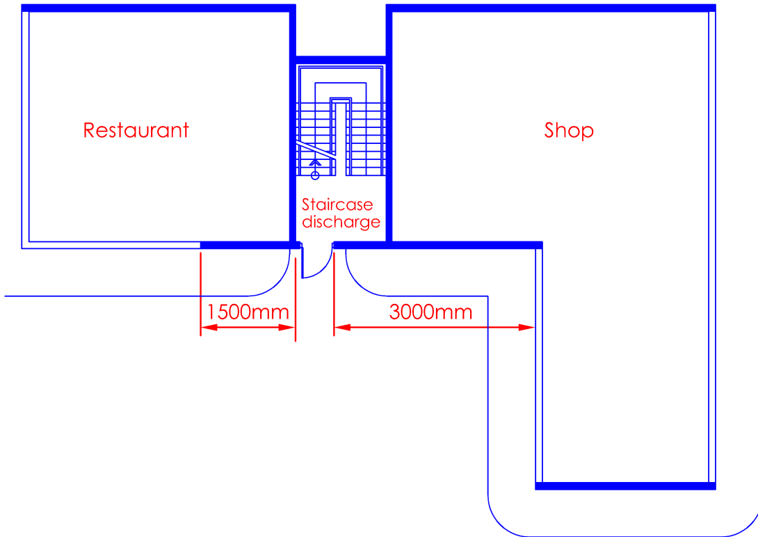
Diagram 2.3.3(c)-(iii)-3
