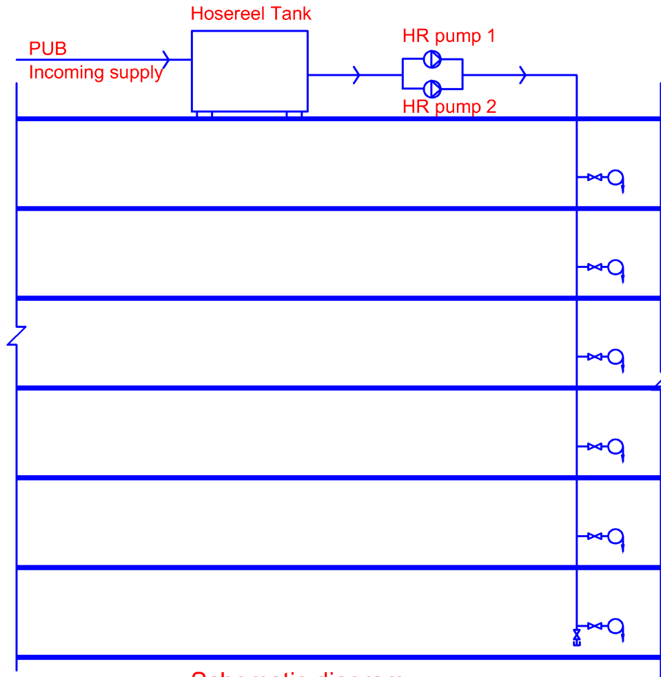
Schematic diagram
