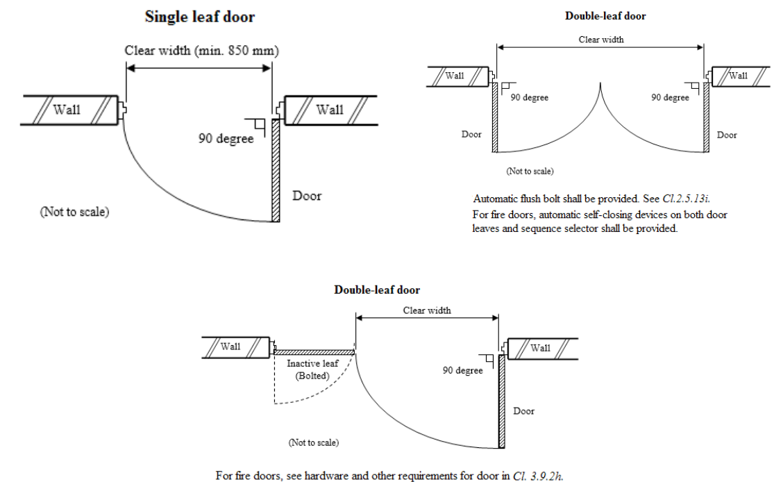
Diagram 2.5.13c. Measurement of door width
