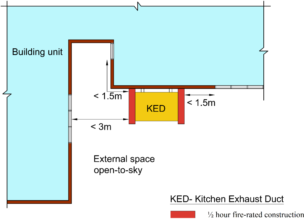
Diagram 7.1.13c.(2) : Fire resistance construction for kitchen exhaust duct
