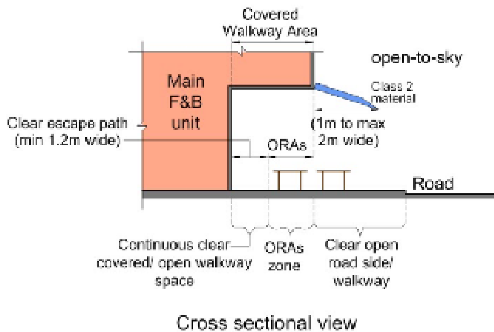
Diagram 9.7.4b.(4)(c) - 1 : ORAs with canopy/awning projection greater than 1m but not exceeding 2m - (without auto retraction)
