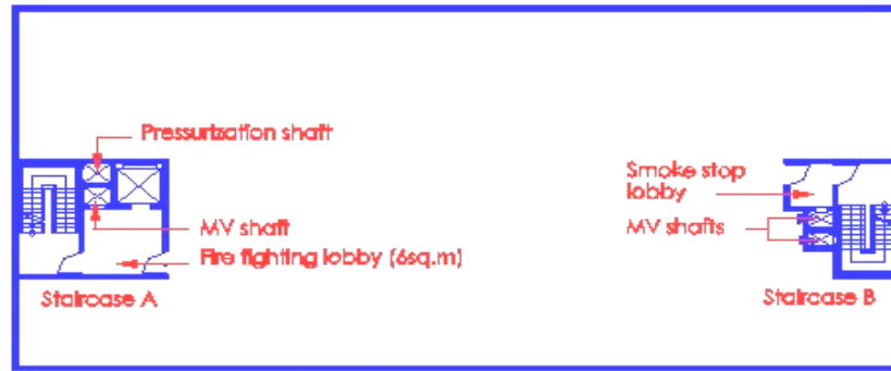
Typical Plan of Basement storey
