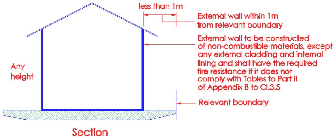
Diagram 3.5.1 – (1)
