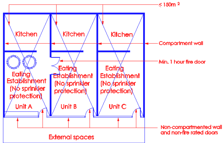
Diagram 3.2.5(f)(v)(d)(ii) – 1
