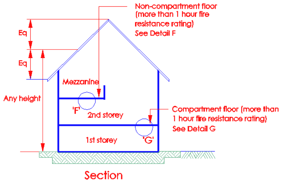
Diagram 3.3.6 - 4
