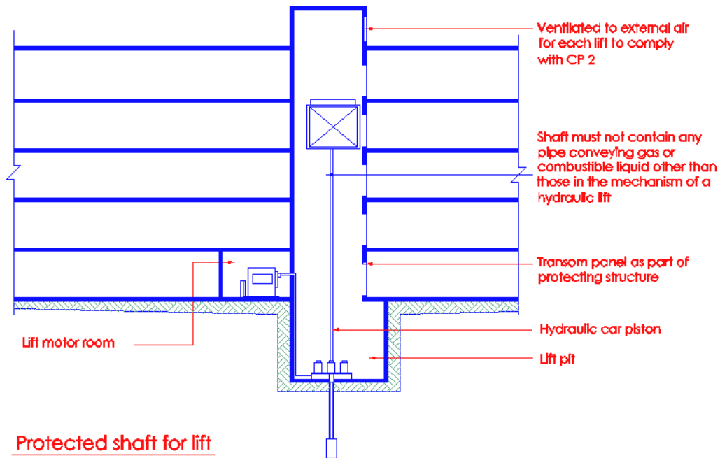
Diagram 3.8.8(a) & (b) - 1
