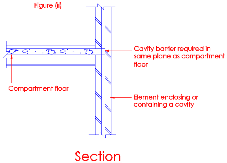
Diagram 3.11.3 – (ii)
