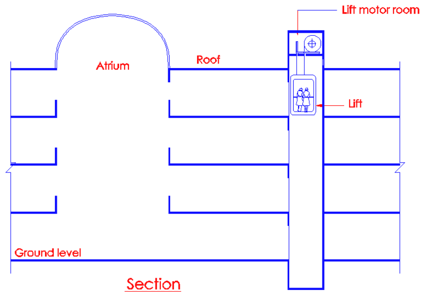
Diagram 3.8.8(c) - 3
