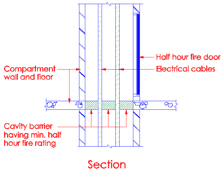
Diagram 3.8.9(b) – (i)
