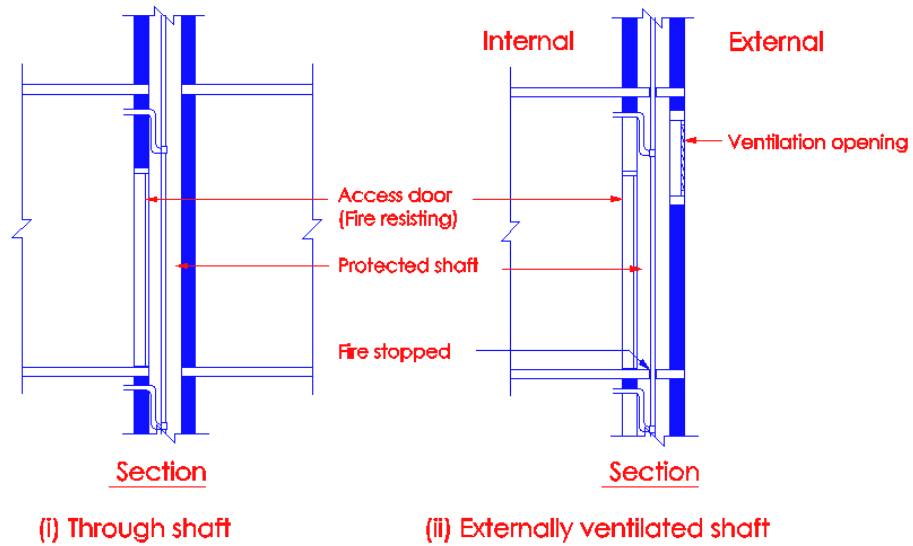
Diagram 3.8.3(c) - 2
