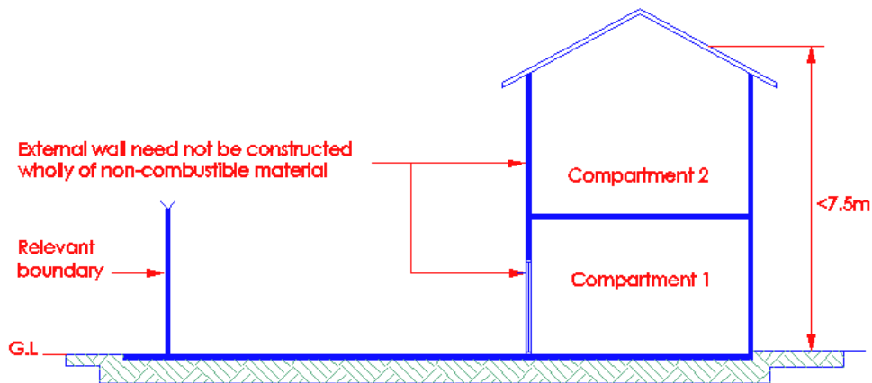
Diagram 3.5.2(b)(iii)
