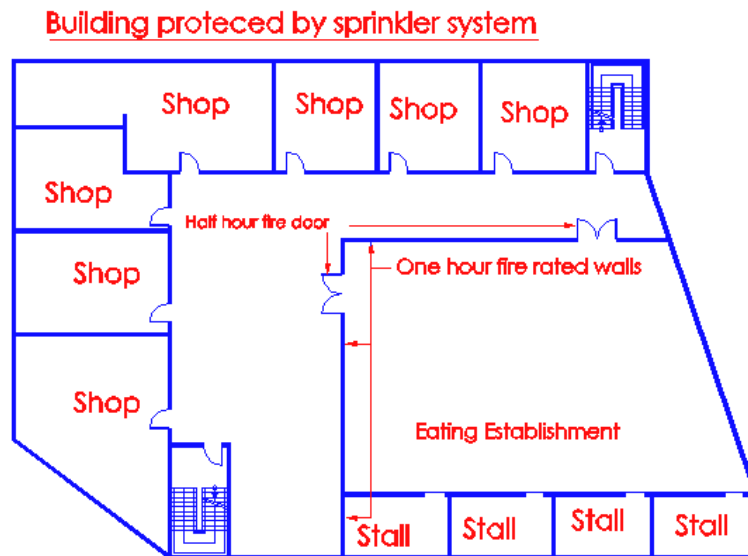
Diagram 3.2.5(f)(v)(d)(II) – 2
