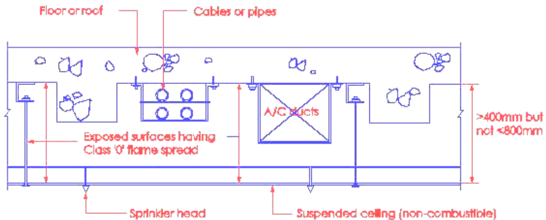
Diagram 3.11.9(e)(ii)
