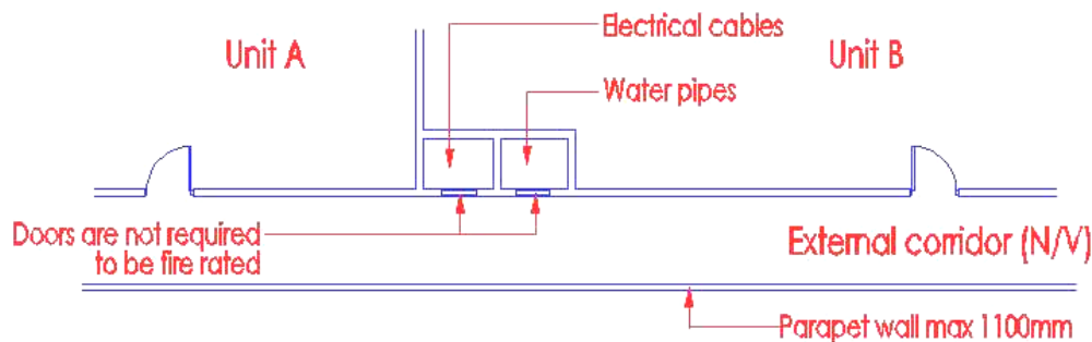
Diagram 3.8.6-2
