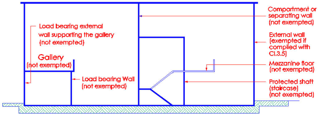
Diagram 3.3.3(b)
