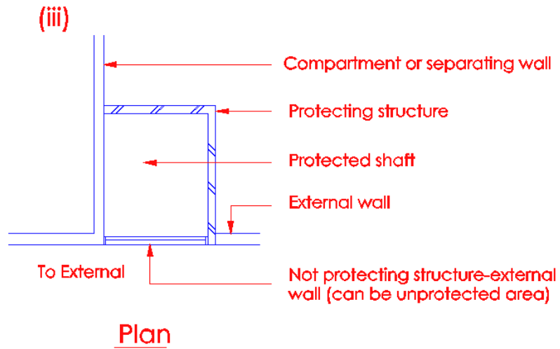
Diagram 3.8.2 - 3
