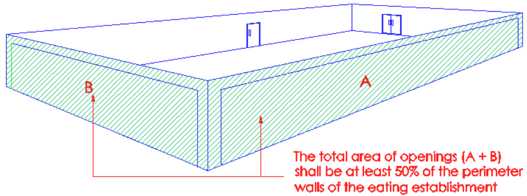
Diagram 3.2.5(f)(v)(c) – 1
