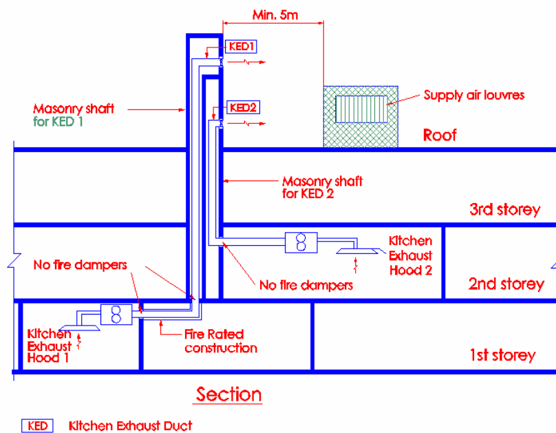
Diagram 3.8.9(a) - 4
