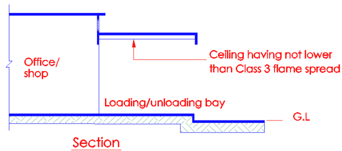
Diagram 3.13.5(b)(iii) - 1
