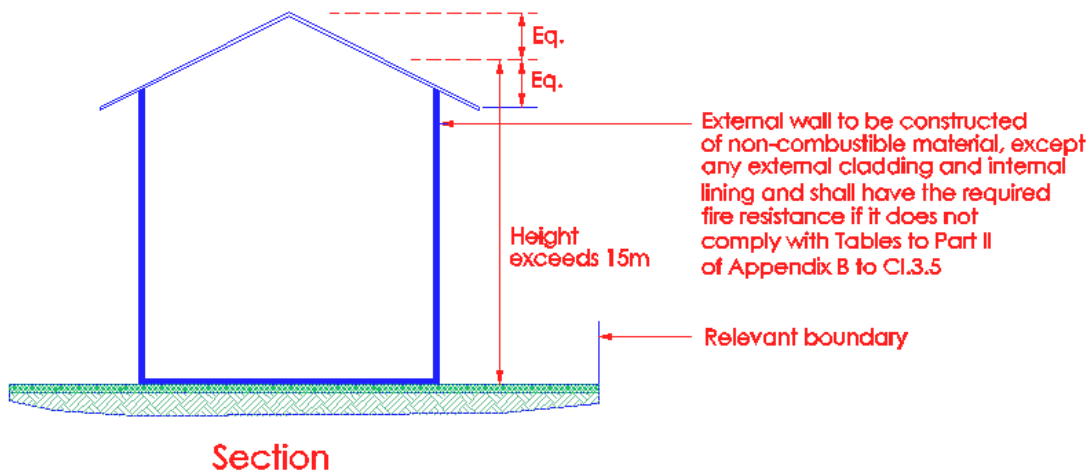
Diagram 3.5.1 – (2)
