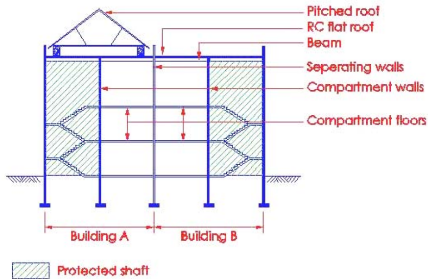
Sectional Elevation
