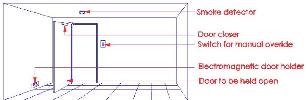
Door is held open position by Electro-magnetic or electro-mechanical device
