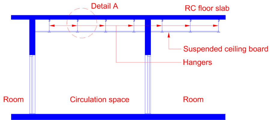
Sectional Elevation
