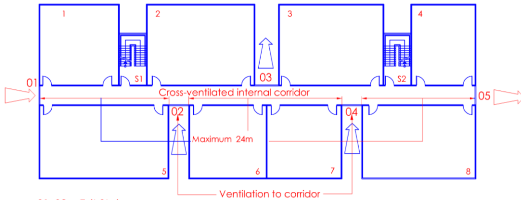
Ventilation of internal corridors to worker's dormitory
