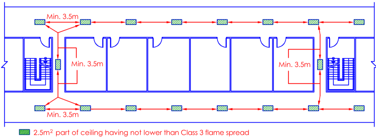
Reflected ceiling plan
