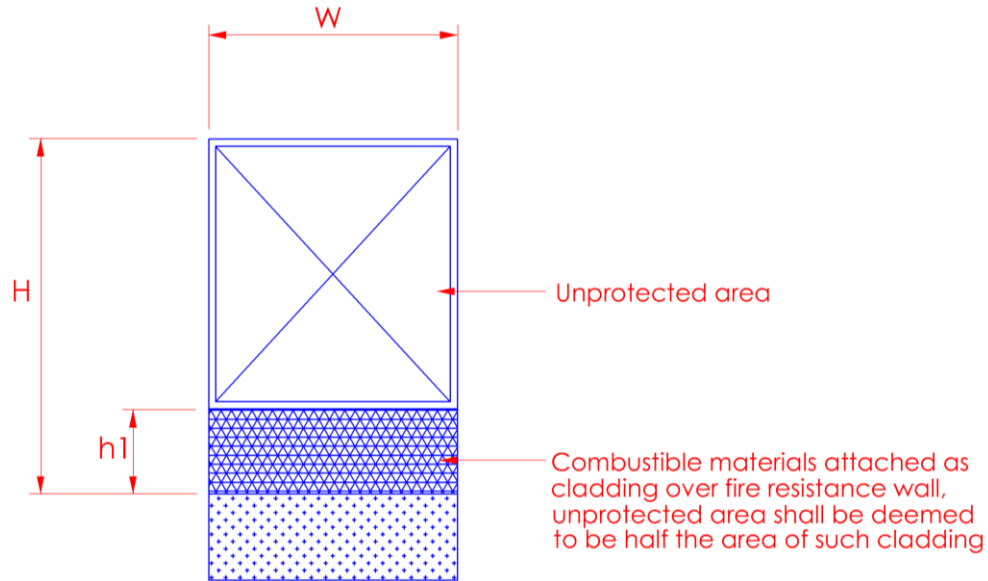
Part Elevation of External Wall
