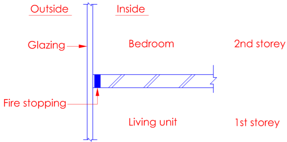
Details at junction of curtain walling at floor
