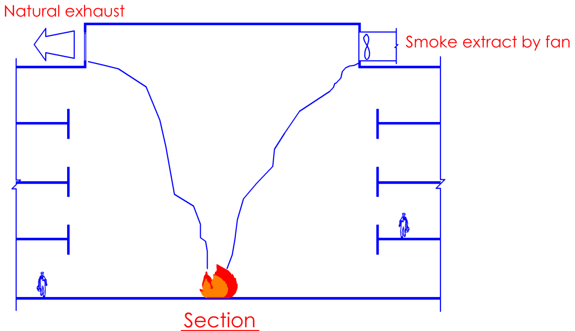
Diagram 7.6.28
