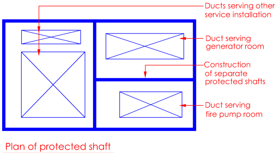
Diagram 7.1.5(c)-2
