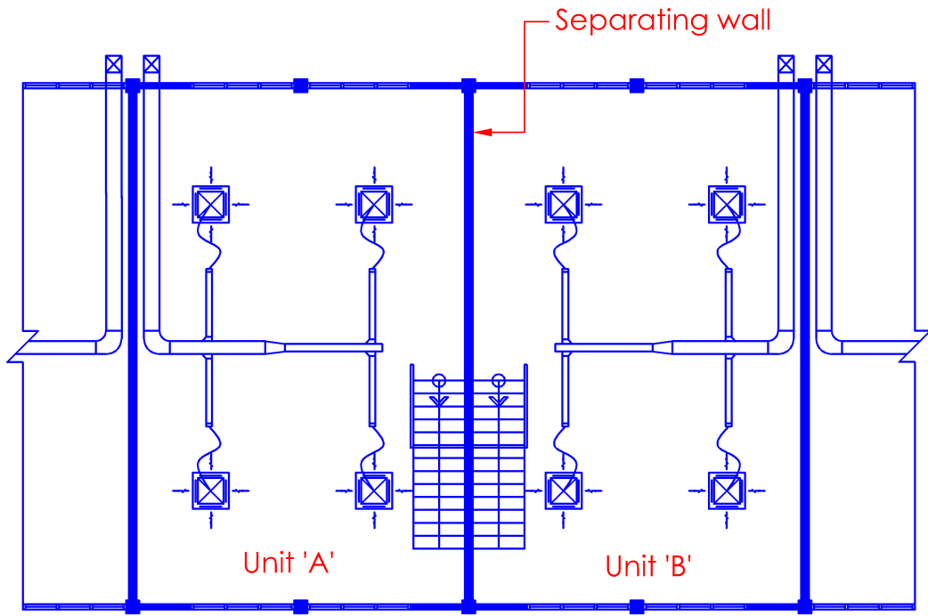
2nd Storey Floor Plan
