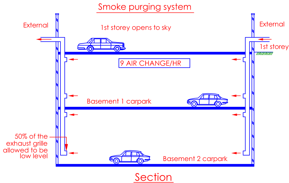
Diagram 7.1.1(h)(iii)
