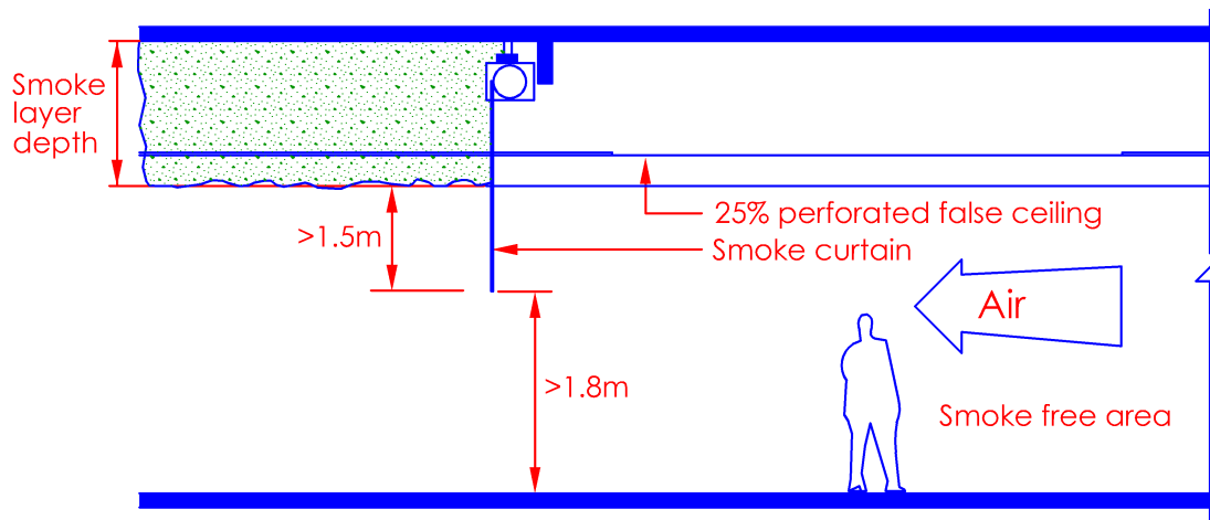
Diagram 7.6.13-1
