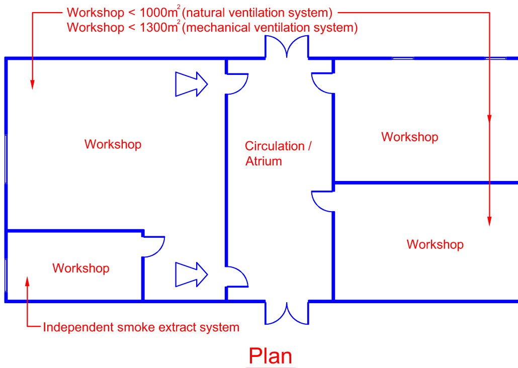
Diagram 7.6.9(a)-1
