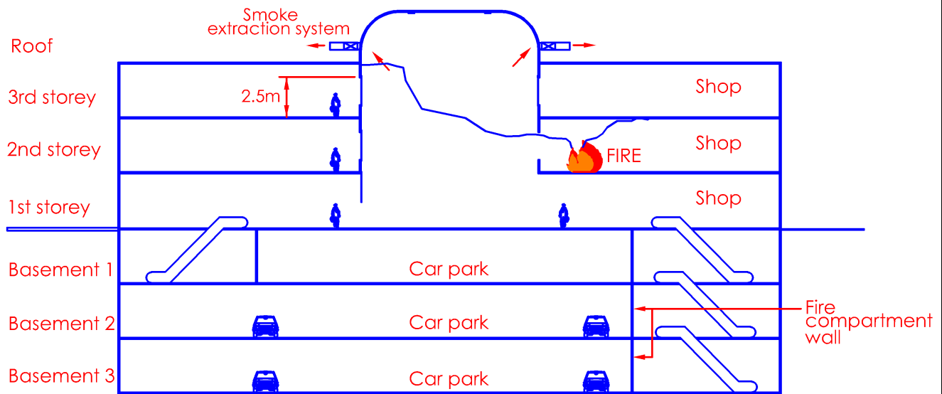
Smoke curtain Section
