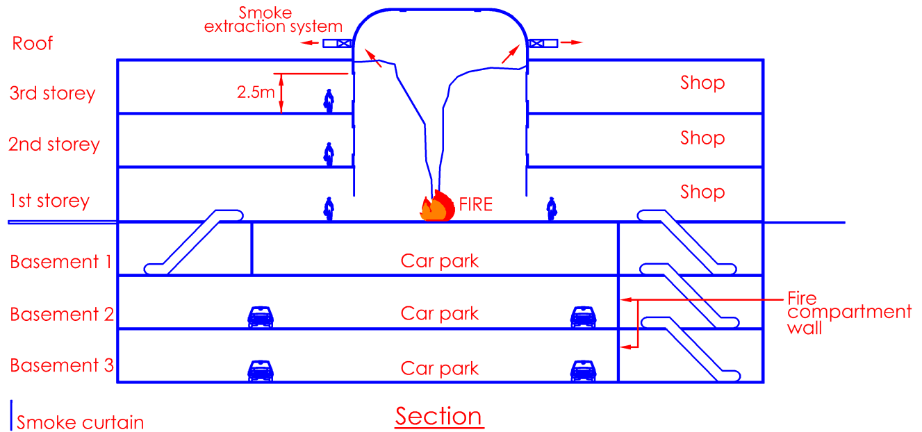
Diagram 7.6.4-1
