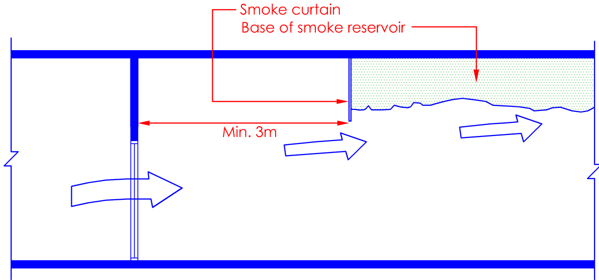
Diagram 7.6.13-3
