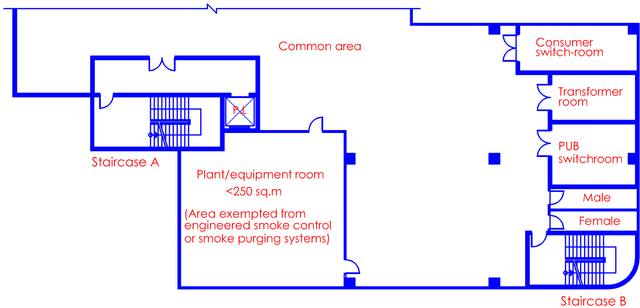
Part plan of basement storey
