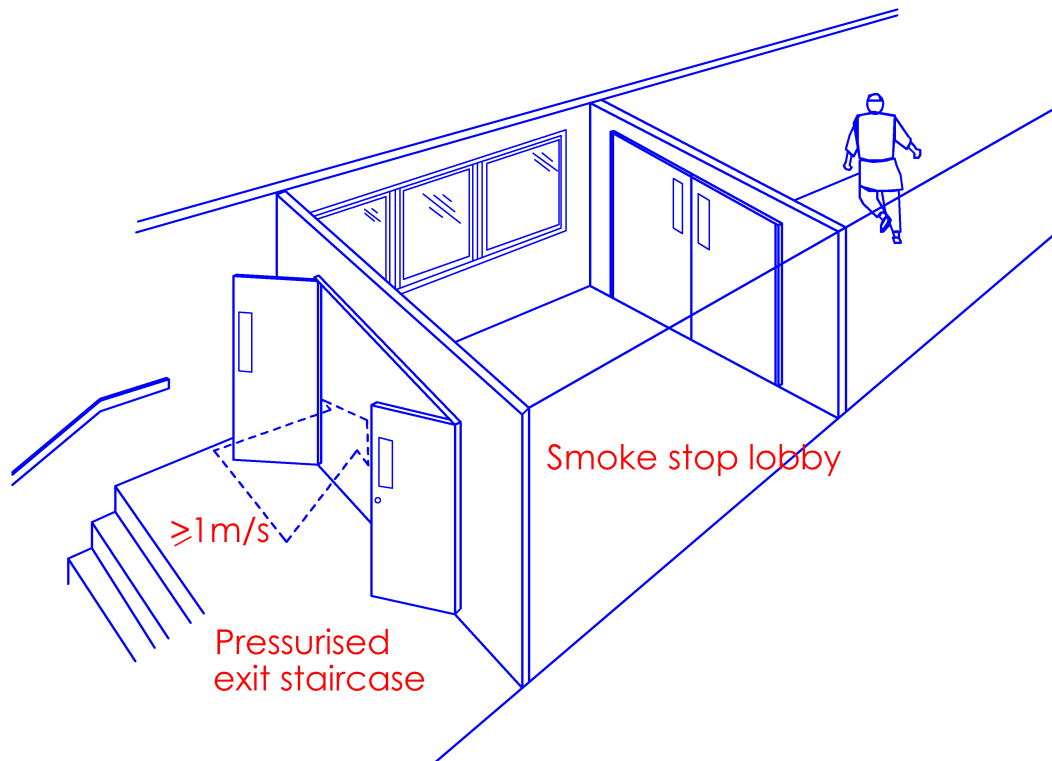
Diagram 7.2.3-2
