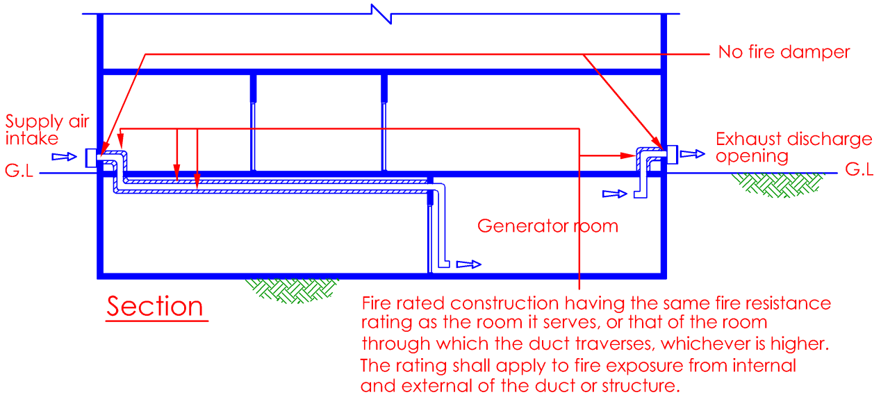
Diagram 7.1.5(c)-1
