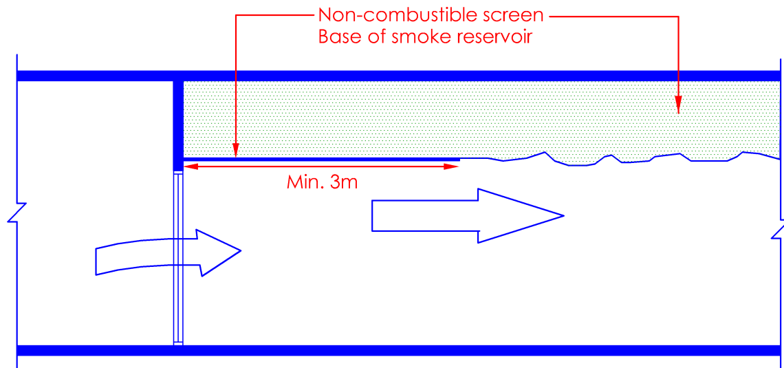
Diagram 7.6.13-4
