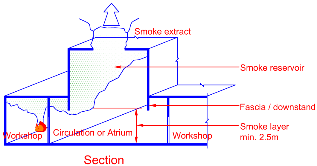
Diagram 7.6.8-1
