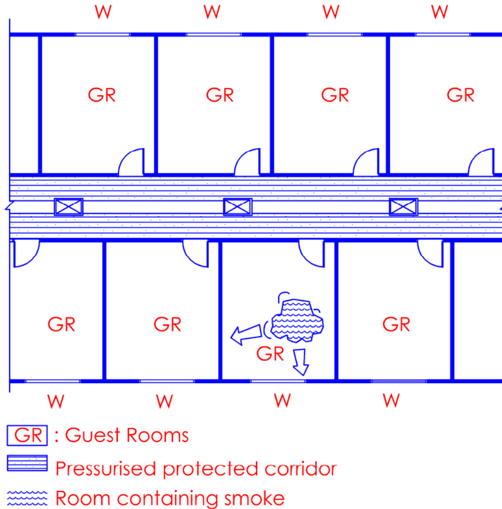
Diagram 7.3.1-7
