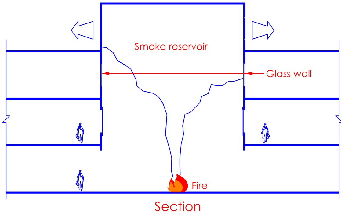
Diagram 7.6.31-1
