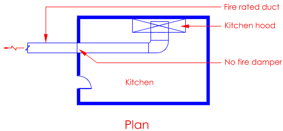
Diagram 7.1.7(a)-2
