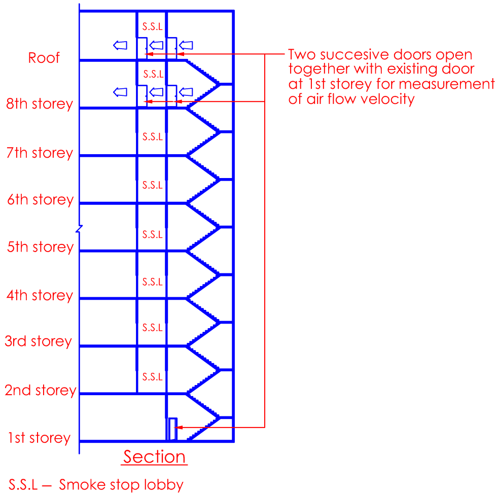
Diagram 7.2.3-1
