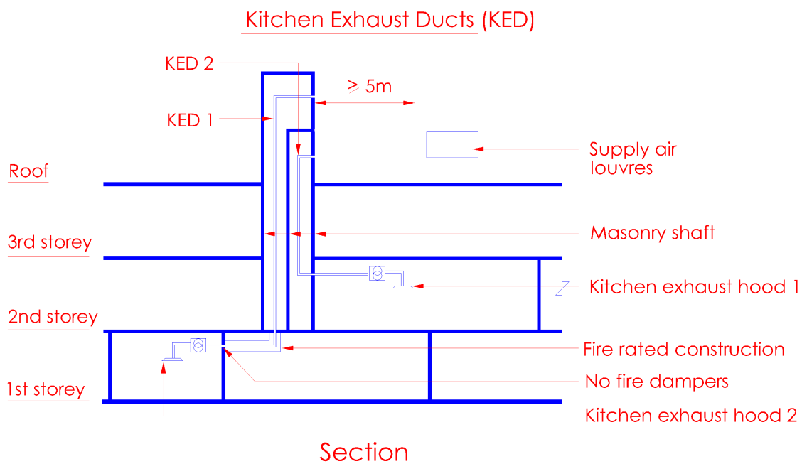
Diagram 7.1.7(a)-1
