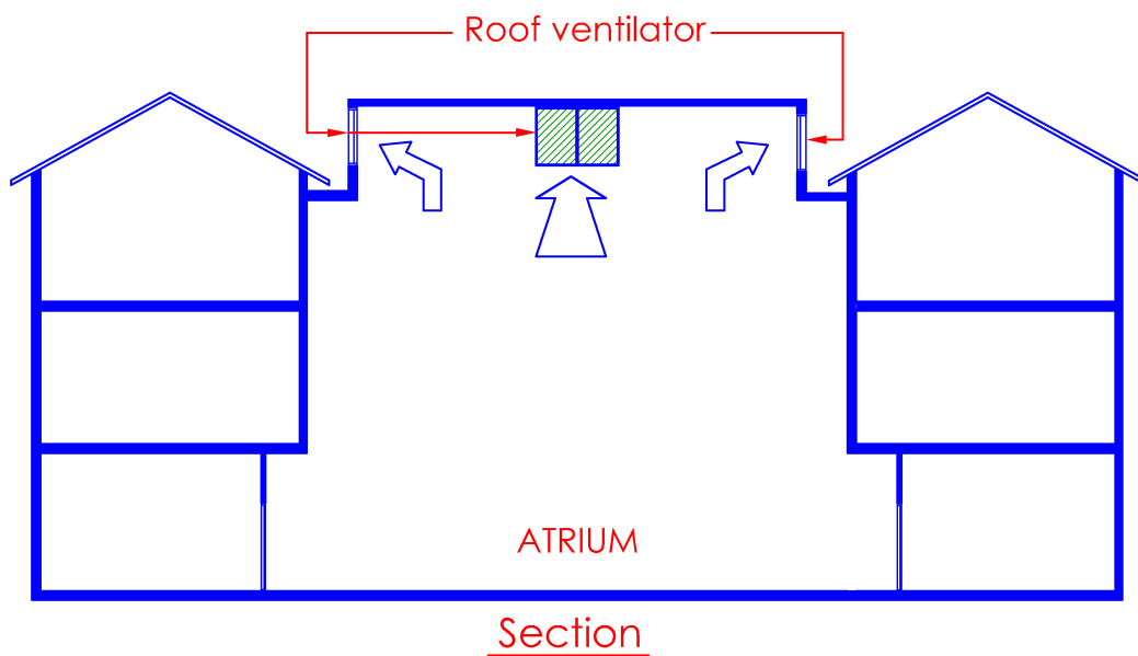
Diagram 7.6.27
