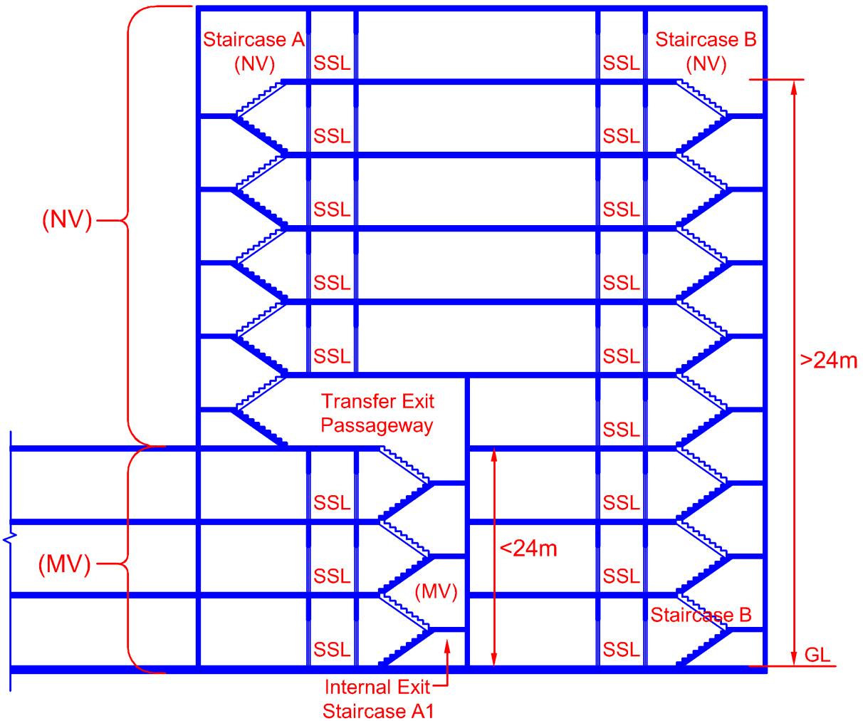
Diagram 7.2.1(a)-2
