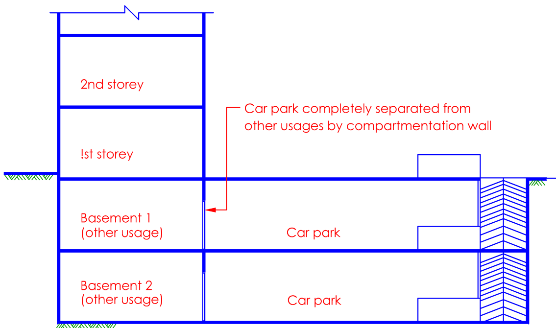
Diagram 7.4.1(b)(i)
