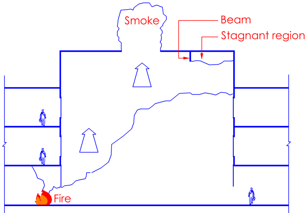
Diagram 7.6.11-2
