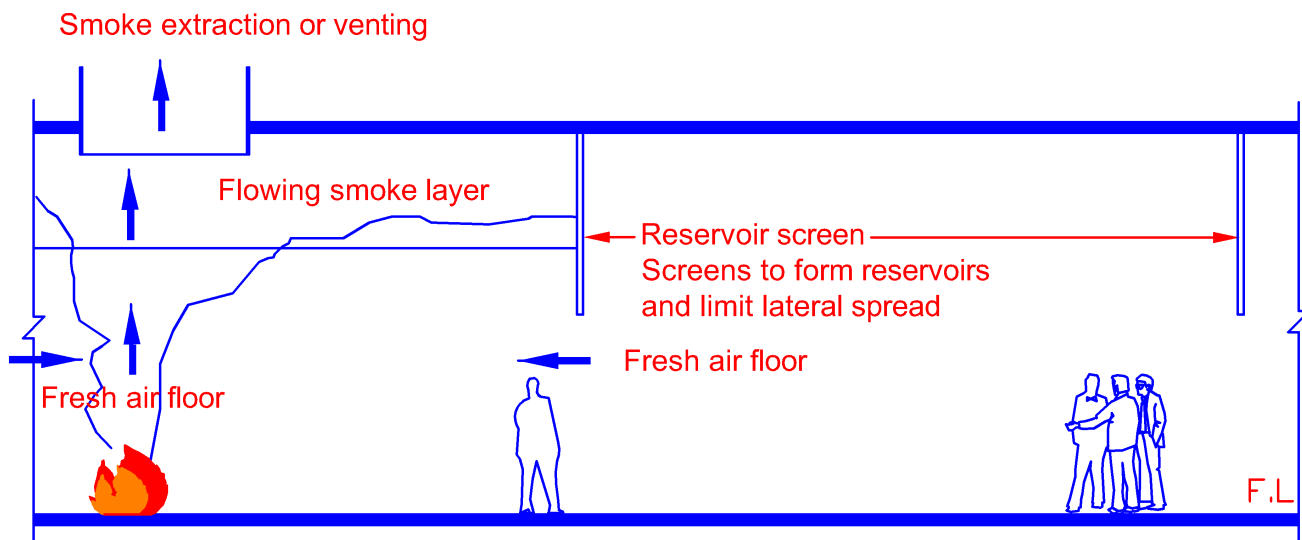
Diagram 7.6.6
