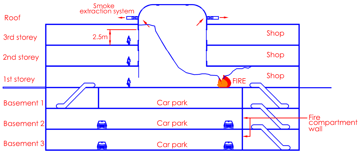
Smoke curtain Section
