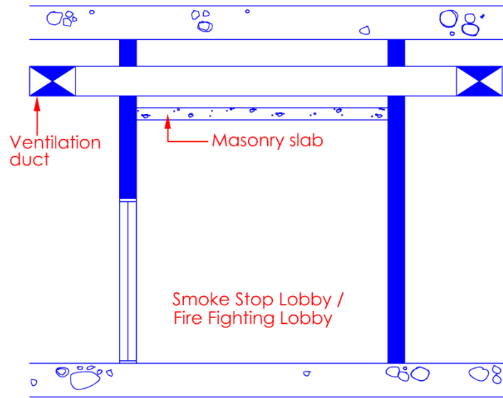
Section
