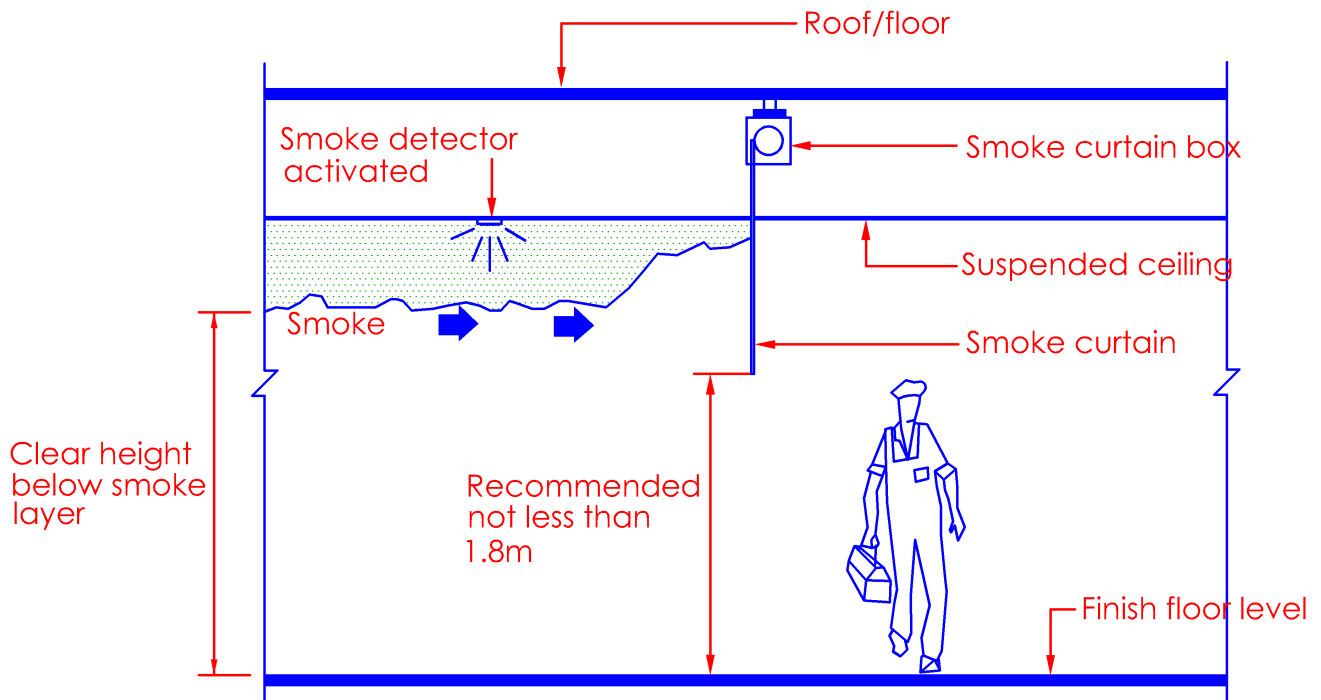
Diagram 7.6.30
