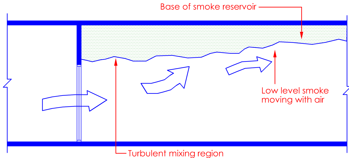
Diagram 7.6.13-2
