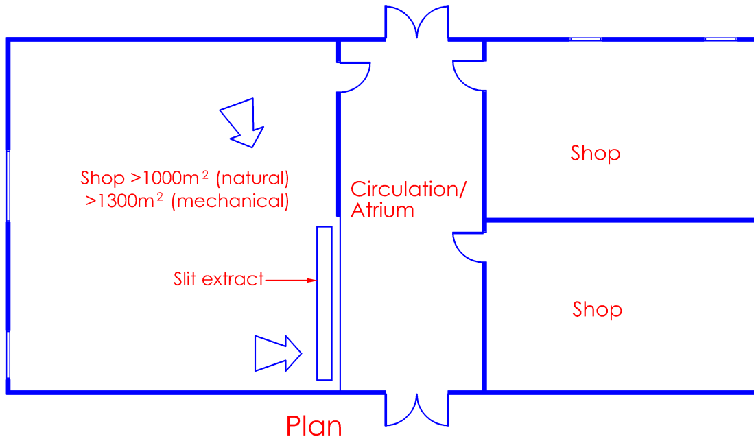
Diagram 7.6.9(b)
