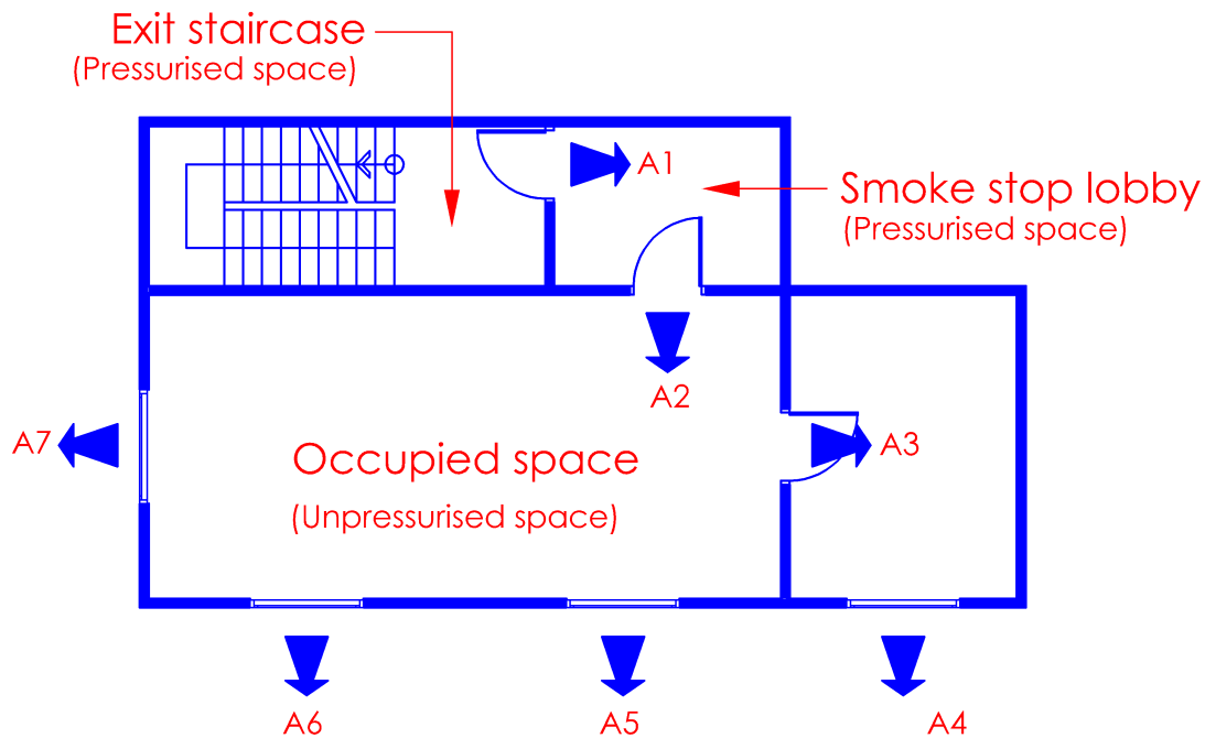
Diagram 7.2.4
