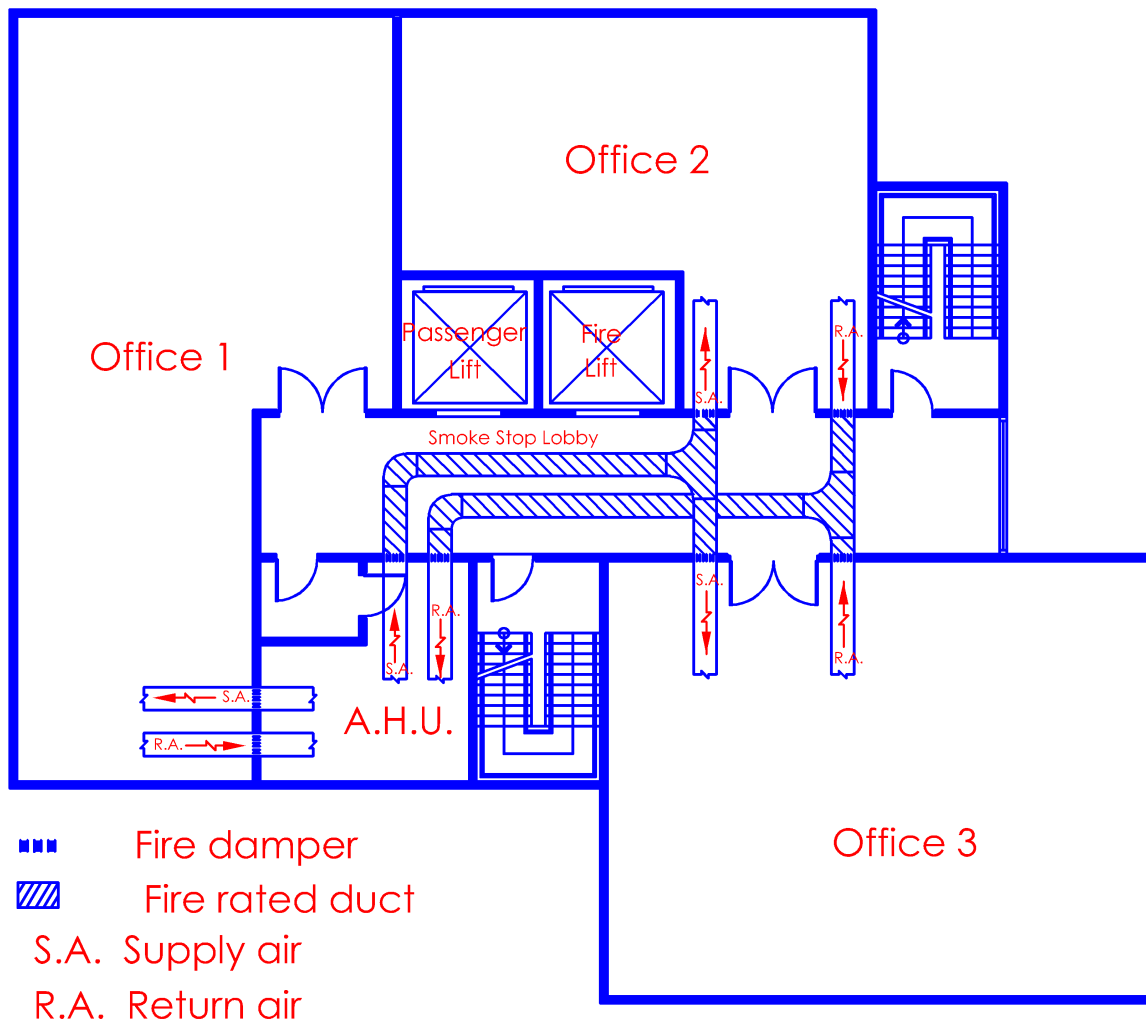
Diagram 7.1.1(e)-4
