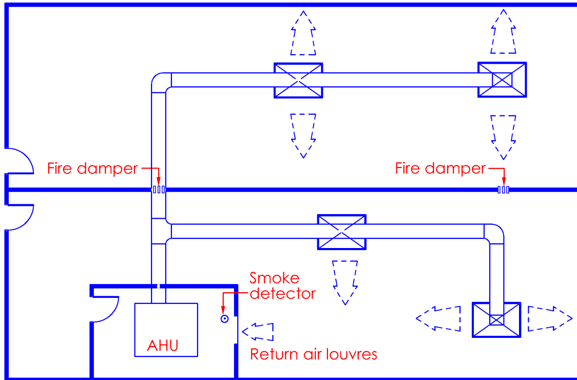
Diagram 7.1.2(a)-1
