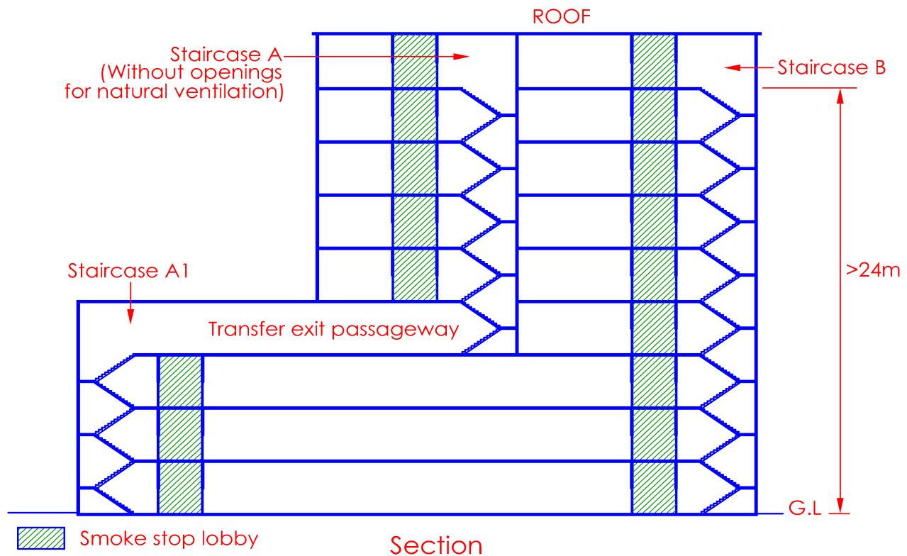
Diagram 7.2.1(a)-5
