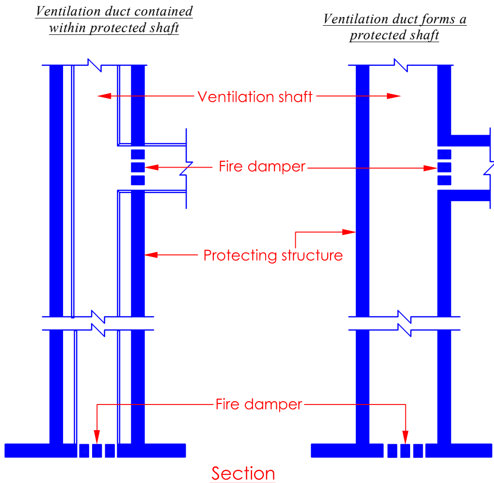
Diagram 7.1.1(h)(i)-2
