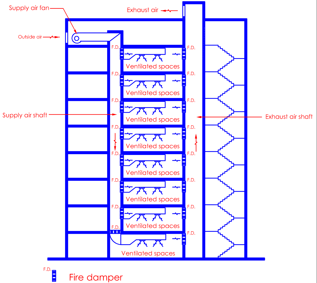
Diagram 7.1.1(h)(i)-3
