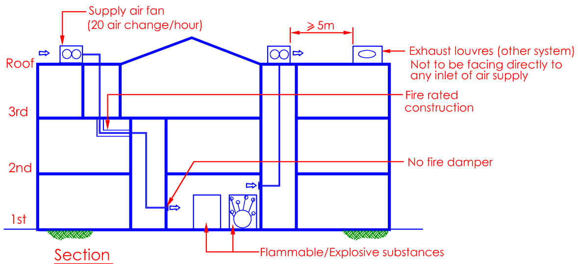
Diagram 7.1.8-1
