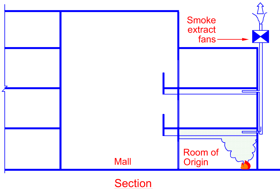
Diagram 7.6.7
