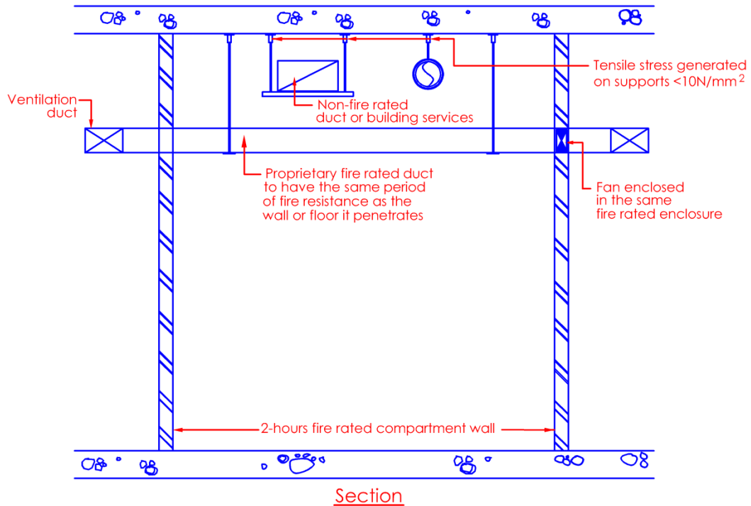
Diagram 7.1.1(j)(iii)
