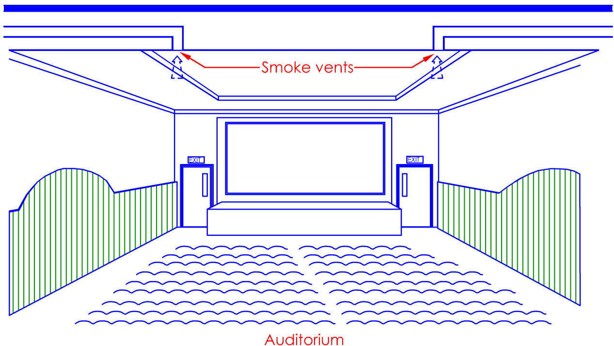
Diagram 7.7.2
