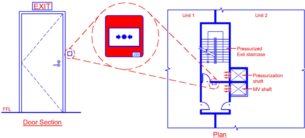
Diagram 7.2.1(c)
