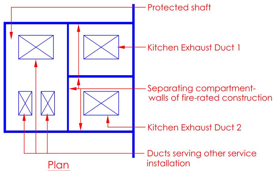
Diagram 7.1.7(a)-3
