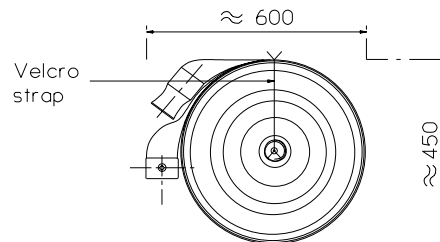
Figure 2 Dutch Roll Folding Method
