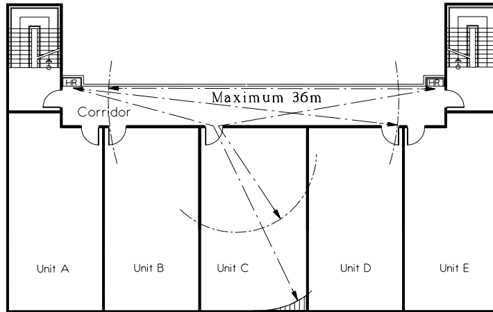
HR Hosereel
